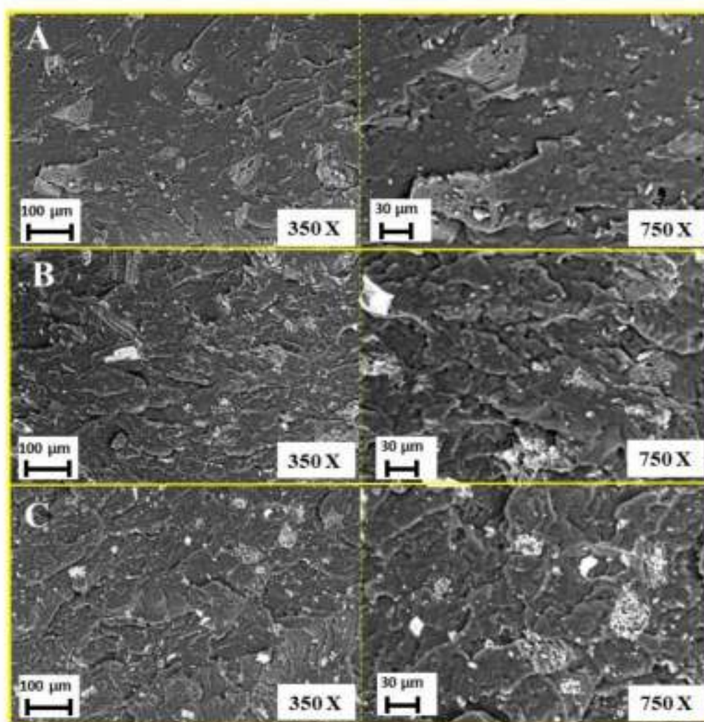
Figure 3. SEM images at different magnification (350 \times and 750 \times ) of EVA + 20 wt% of: BC low (A); BC medium (B); and BC high (C).
