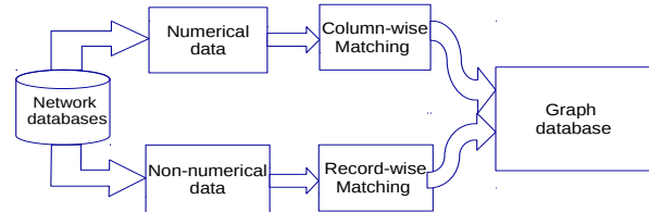
Fig. 2: System diagram of automatic integration for network management databases.
