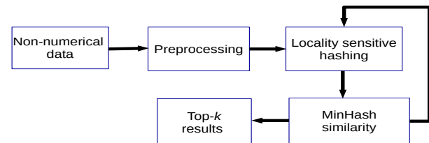
Fig. 5: Non-numerical field matching flow based on MH-LSH.
