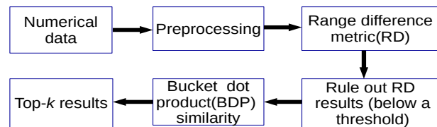
Fig. 3: Numerical field matching flow.
