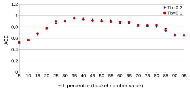
Fig. 8: Selection of the best T_b based on the matching accuracy.
