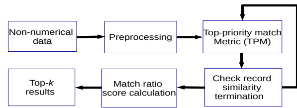
Fig. 4: Non-numerical field matching flow based on TPM.
