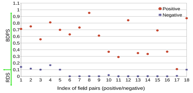
Fig. 7: Matching with combined RDS and BDPS 1 .
