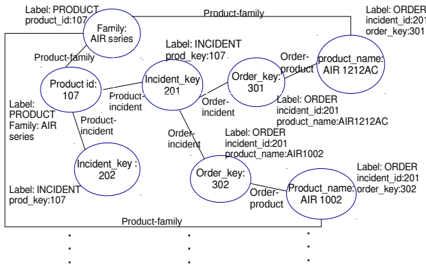
Fig. 1: Graph database created from Table I, II and III.
