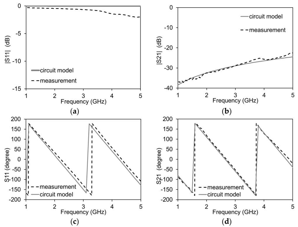
Figure 12. Simulated (solid lines) and measured (dashed lines) scattering parameters of gap: (a) amplitude of reflection coefficient (dB); (b) amplitude of transmission coefficient (dB); (c) phase of the reflection coefficient (deg); (d) phase of the transmission coefficient (deg).
