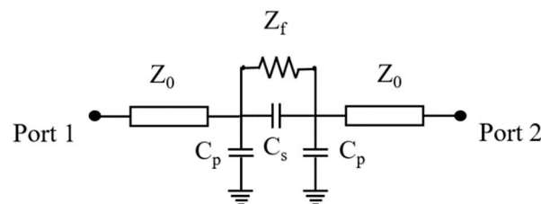
Figure 3. Circuit model representation of the microstrip line with gap including film.
