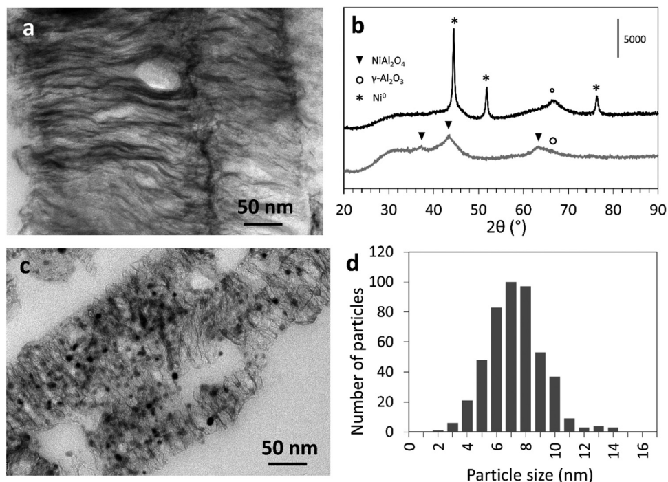
Fig. 3 (a) TEM image of a microtome cut of \text{Ni}-\text{Al}_2\text{O}_3\text{-PET} , (b) PXRD patterns of \text{Ni}-\text{Al}_2\text{O}_3\text{-PET} (grey line, bottom) and of \text{Ni}^0\text{-Al}_2\text{O}_3\text{-PET} (black line top), (c) TEM image of a microtome cut of \text{Ni}^0\text{-Al}_2\text{O}_3\text{-PET} and (d) histogram established from at least 450 \text{Ni}^0 nanoparticles in typical TEM images of \text{Ni}^0\text{-Al}_2\text{O}_3\text{-PET} .
