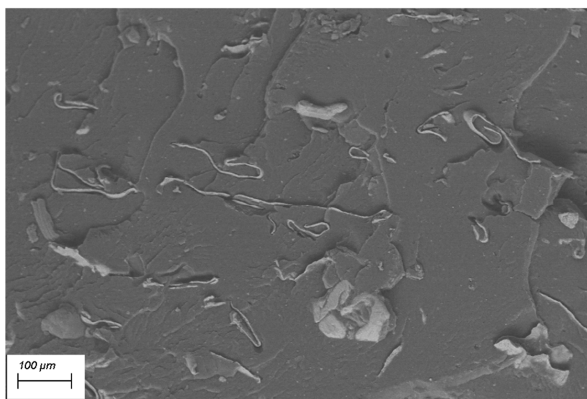
Figure 2. SEM image 250× of compression-moulded PEAL.
