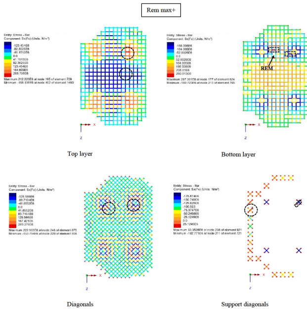
Figure 10: Stress contour plots after most tensile bar removal for LC 1 (red = tension; blue = compression)
