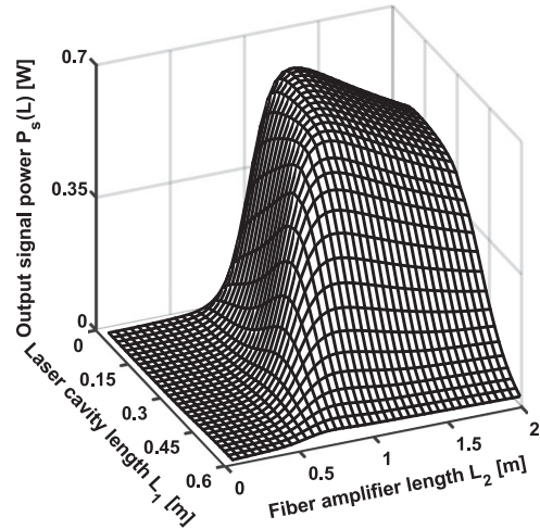
Fig. 8. Output signal power P_s(L) of the Dy 3+ -doped MOPA versus laser cavity length L_1 and fiber amplifier length L_2 . Input pump power P_p(0) = 3 W; dopant concentration N_{Dy} = 6 \times 10^{25} ions/m 3 ; first mirror reflectivity R_1 = 99\% ; second mirror reflectivity R_2 = 70\% .
