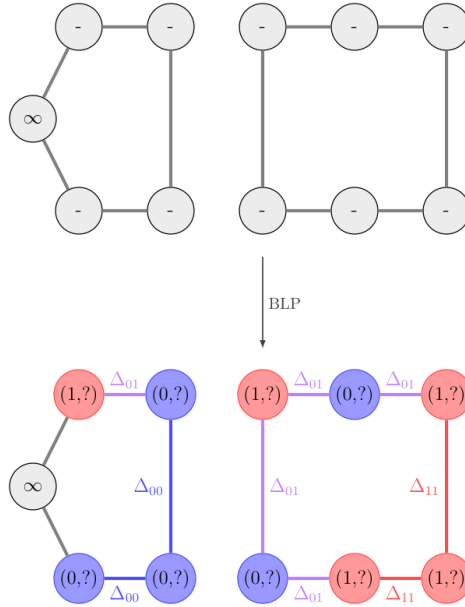
Figure 5: (BLP) over OP(F = [5, 6]) .
