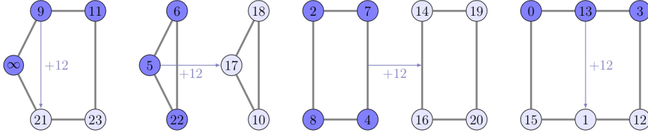
Figure 4: F instance derived from F^* = [3_\infty, 3, 4, 3_c] .
