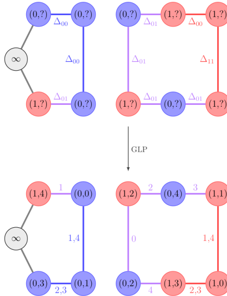
Figure 6: (GLP) over OP(F = [5, 6]) .
