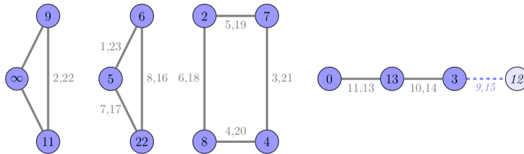
Figure 3: F^* instance for F = [5,^2 3,^2 4, 6] .
