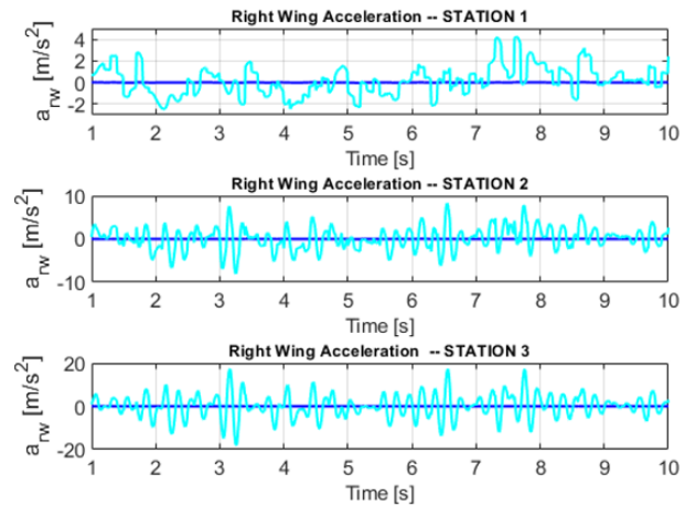
Figure 6. Bending Accelerations (von Kármán)
