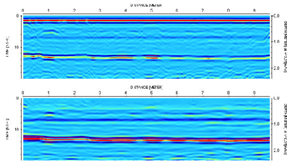
Fig. 7: Site Broussailles-Profile 2-top) raw radar data collected using a central frequency of 900 MHz, bottom) filtered and migrated image
