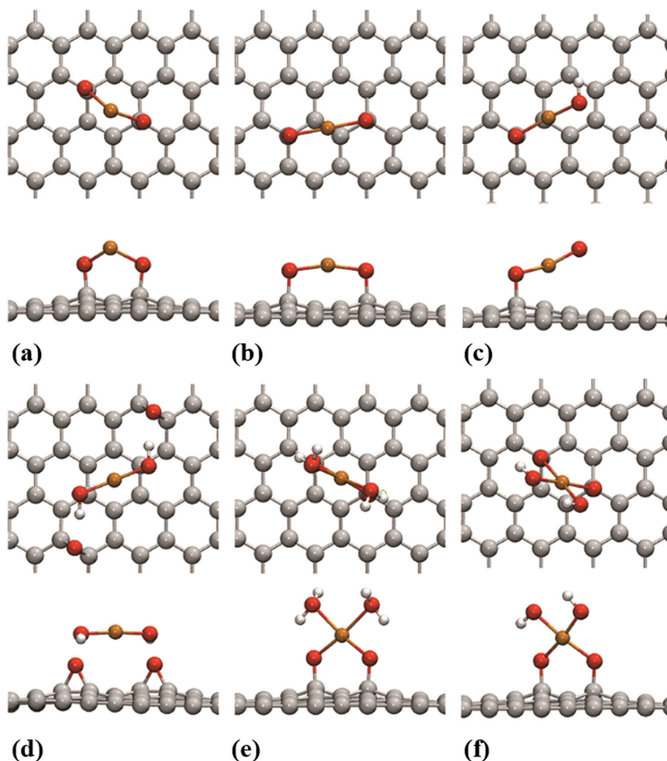
Fig. 3 Ball and stick representation of Cu-N-rGO structures. a, b Cu ion is coordinated to two surface -\text{O}^- groups, c Cu ion is coordinated to one surface -\text{O}^- group and also bound to one hydroxyl group, d Cu ion is coordinated to two surface epoxide groups, e, f Cu ion is coordinated to two surface -\text{O}^- groups and also bound to hydroxyl groups. Gray spheres represent C atoms, red spheres O atoms, white spheres H atoms and orange spheres Cu atoms.
