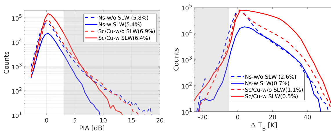
Figure 10. PIA (left) and \Delta T_B (right) pdfs for snowy profiles for different snow cloud types (Ns and Sc+Cu) and with or without SLWC at cloud top. The percentage in the bracket in the legend of the two panels represents the percentage exceeding the 3 dB threshold and -5 K threshold, respectively, as indicated by the shaded grey regions.
