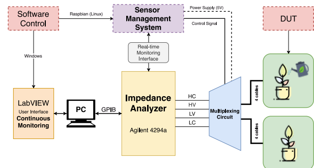
Fig. 1. Full system architecture showing impedance measurements and environment sensors connection
