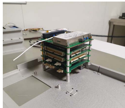
Figure 1. View of the Avionics box.
