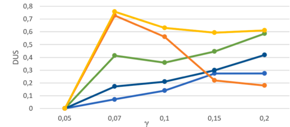
Fig. 4. Average DUSV and DUS for uniform datasets under the exploratory plan.
