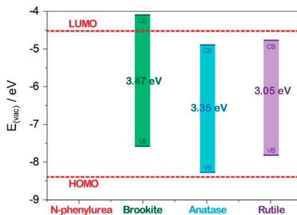
Scheme 3. Position of the calculated VB and CB of pure brookite, anatase and rutile TiO 2 polymorphs. [54] The calculated HOMO and LUMO values of NPU are reported for the sake of completeness. [55]
