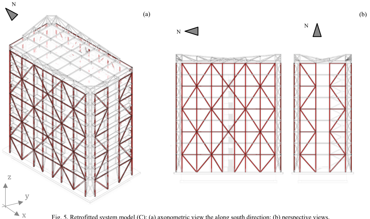
Fig. 5. Retrofitted system model (C): (a) axonometric view the along south direction; (b) perspective views.
