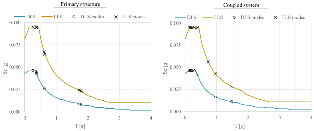
Fig. 7. Horizontal component of elastic pseudo-acceleration response spectra of both structural systems.
