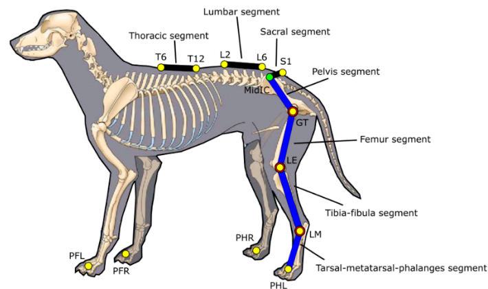
Figure 1. Marker-set of 17 retro-reflective spherical markers attached to selected ALs; the multi-segmental model included 10-line segments including three segments for modeling the back (sacral segment, lumbar and thoracic segments). Tarsus, stifle and hip joints are modeled as spherical hinges.
