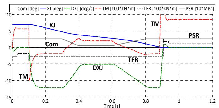
Figure 7 Reversible mechanical subsystem retraction.
