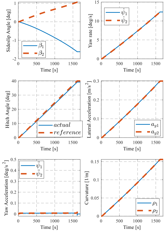
Figure 11. Ramp hitch angle at 5 km/h and \mu = 0.8 : sideslip angle, yaw rate, hitch angle, lateral acceleration, yaw acceleration and curvature for both modules.
