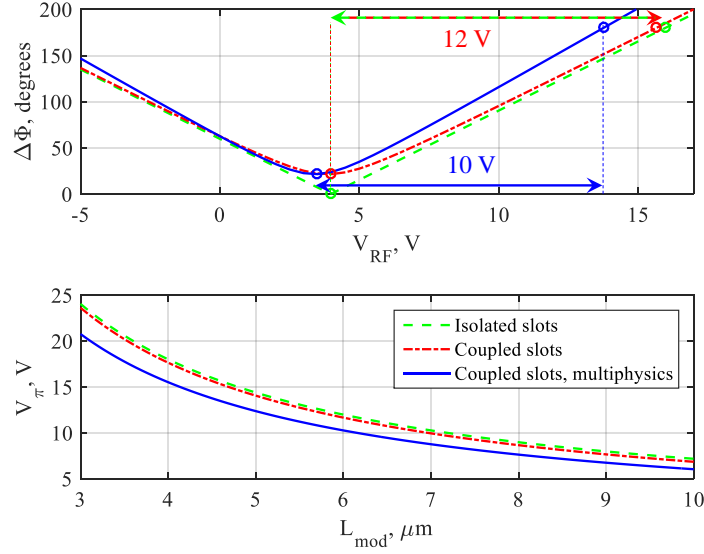
Fig. 5. Top: \Delta\Phi(V_{RF}) characteristics evaluated with (5) using the waveguide simulations shown in Fig. 3, assuming L_{mod} = 6 \mu\text{m} . The green dashed, red dash-dotted and blue solid curves are obtained considering the slots isolated, coupled, and coupled including multiphysics effects, respectively. The horizontal arrows indicate the V_\pi definitions for the three simulations. Bottom: the curves show the behaviour of V_\pi versus L_{mod} using the definition indicated in the top panel.
