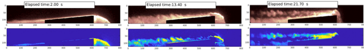
Fig. 18 Naphthalene fluorescence signal (above) and fluctuations about the mean (below) for a capsule model at 0^\circ angle of attack
