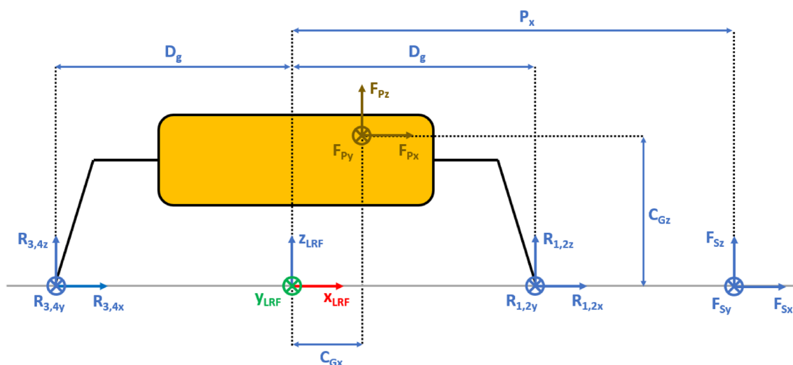
Fig. 8 Free body diagram and main geometric parameters (XZ plane view) for the 4-legged lander. Qualitative scheme, not to scale
