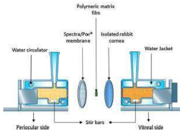
Figure 4. Side-by-Side Diffusion Apparatus Setup
