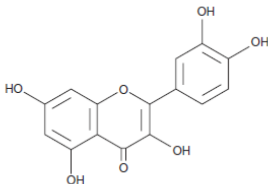
Figure 3. Quercetin Structure
