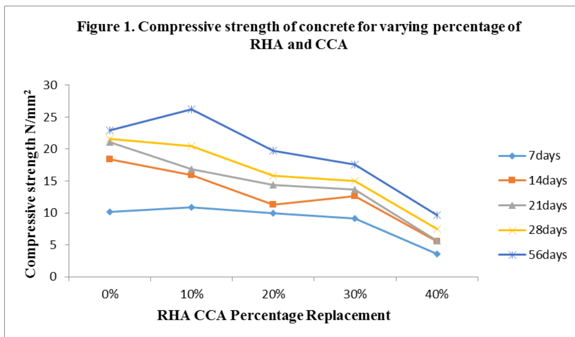
Figure 1. Compressive Strength of Concrete for Varying Percentage of RHA and CCA
