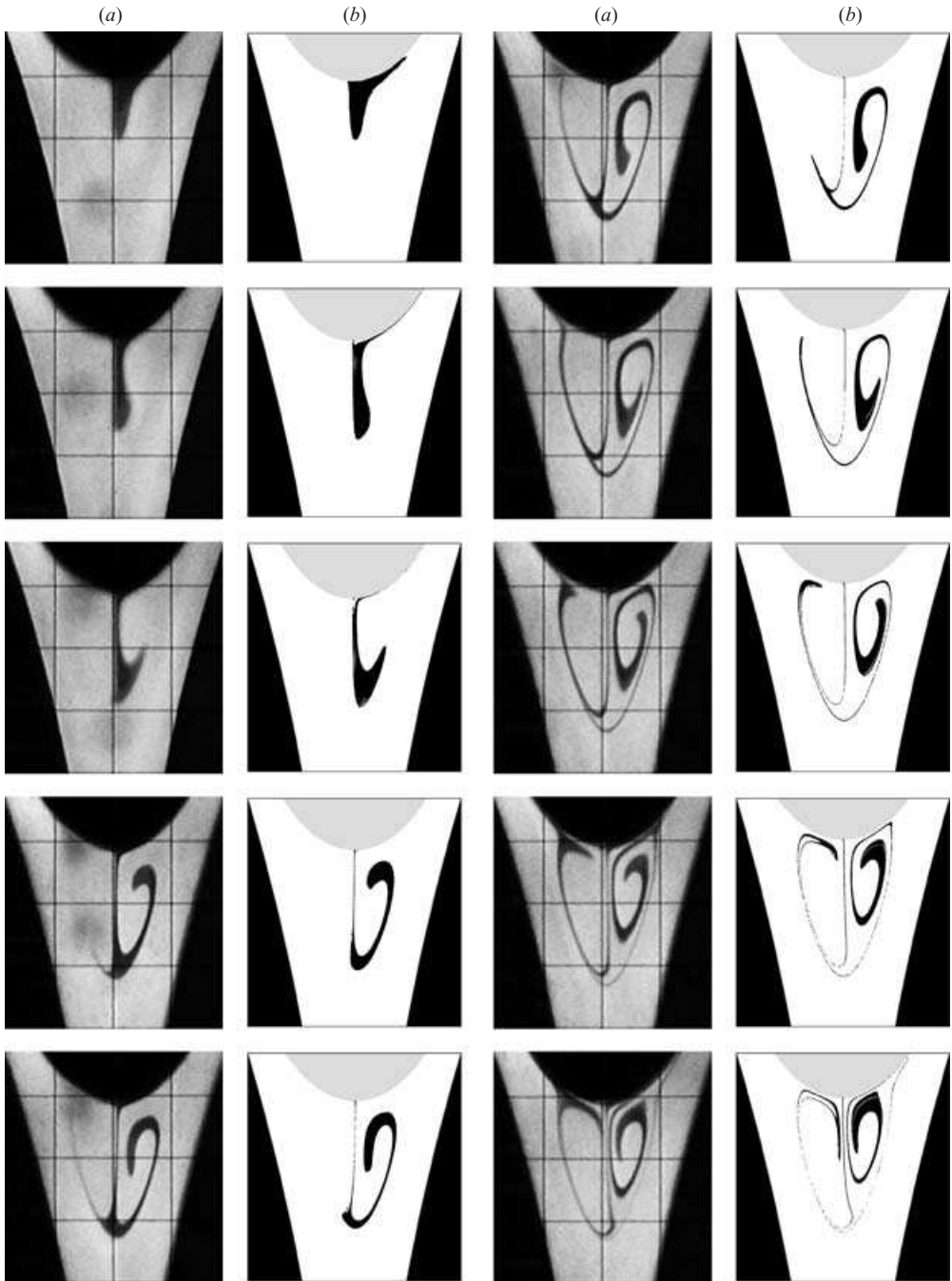
FIGURE 7. Comparison of simulation (b) with experiment (a) for the evolution of a dye blob dropped onto the free surface. Time increases in steps of 1 s in the vertical sense. The period of modulation is 10.57 s, so the images illustrate a little under one period. The phase in the top left image is 0.78, and the Hooke's joint is set at 30^\circ with \bar{S} = 1 , giving the range 0.866 \leq S \leq 1.154 .
