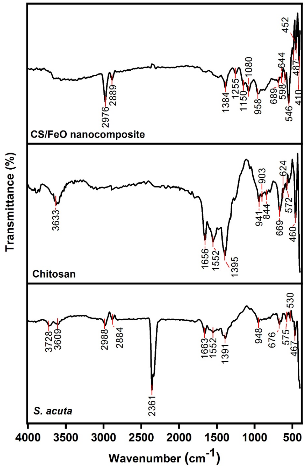
Figure 3. FTIR spectra of CS/FeO NC, CS, and S. acuta leaf extract in a wavenumber range of 500–4000 cm -1 .
