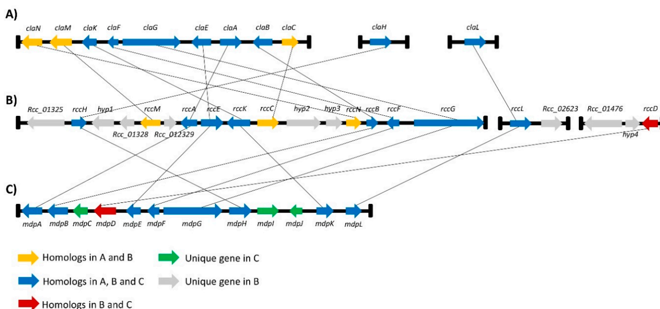
Figure 3. Homology between the rubellin candidate cluster and gene clusters involved in the biosynthesis of known secondary metabolites structurally related to rubellin; (A) The cladofulvin biosynthetic gene cluster in C. fulvum was described by Griffith et al.; (B) The rubellin candidate gene cluster in R. collo-cygni consists of gene clusters organised around the core gene rccG as well as two miniclusters named rccL - and rccD miniclusters organised around rccL and rccD , respectively; (C) The monodictyphenone biosynthetic gene cluster in A. nidulans was identified by Chiang et al. [42]. Homology was confirmed by reciprocal BLAST using the NCBI database.
