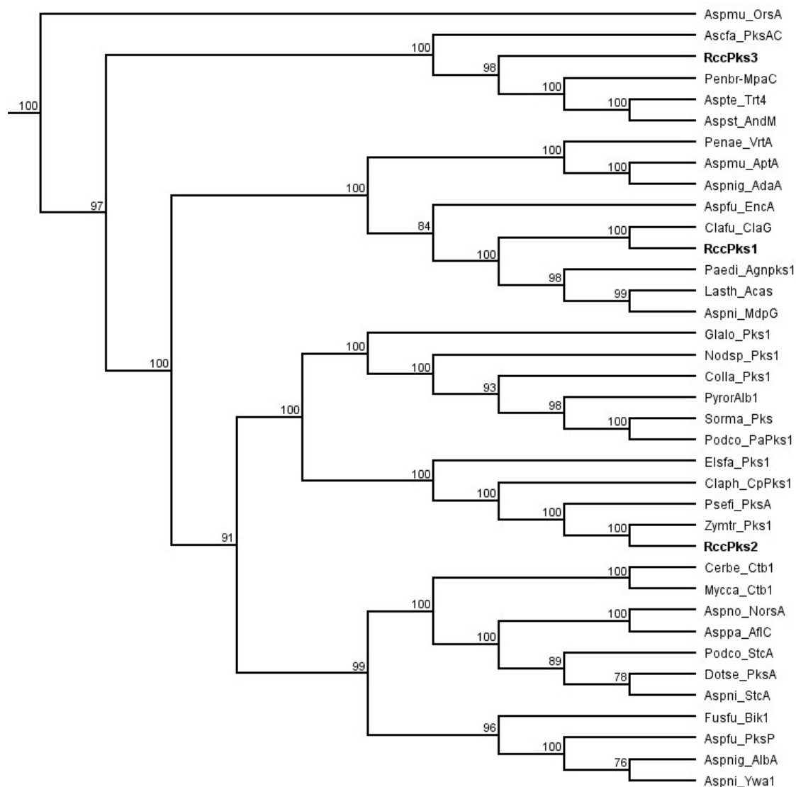
Figure 2. Phylogenetic analysis of R. collo-cygni nonreducing polyketide synthases (NR-PKSs). The cladogram was obtained using maximum likelihood on full-length protein sequences with 100 replications and nodal support value cutoff set at 75%. The list of sequences used in this study can be found in Supplementary information Table S1.
