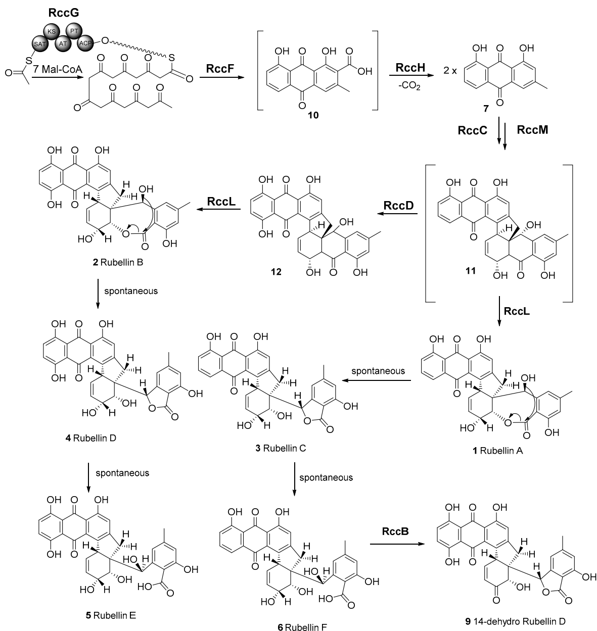
Figure 6. Proposed biosynthetic pathway of rubellins A–F (1–6) and 14-dehydro rubellin D 9. RccG—nonreducing, iterative type I polyketide synthase (PKS). PKS domains: ACP—acyl carrier protein; PT—product template; AT—acyl transferase; KS—keto synthase; SAT—starter unit acyl carrier protein transacylase; RccF—β-lactamase; RccH—decarboxylase; RccC—short-chain reductase; RccM—cytochrome P450; RccD—FAD-dependent monooxygenase/hydroxylase; RccL—Baeyer–Villiger monooxidase; RccB—dehydratase.
