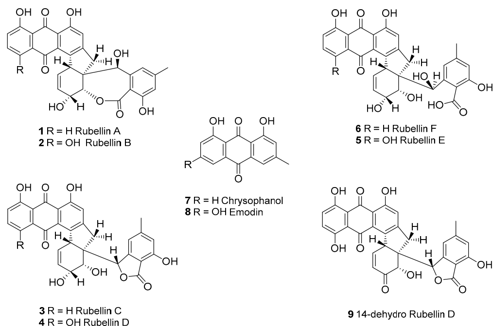
Figure 1. Structures of the rubellins A–F (1–6), chrysophanol 7, the possible precursor of the rubellins and emodin 8, its analogue, as well as the 14-dehydro rubellin D derivative 9.
