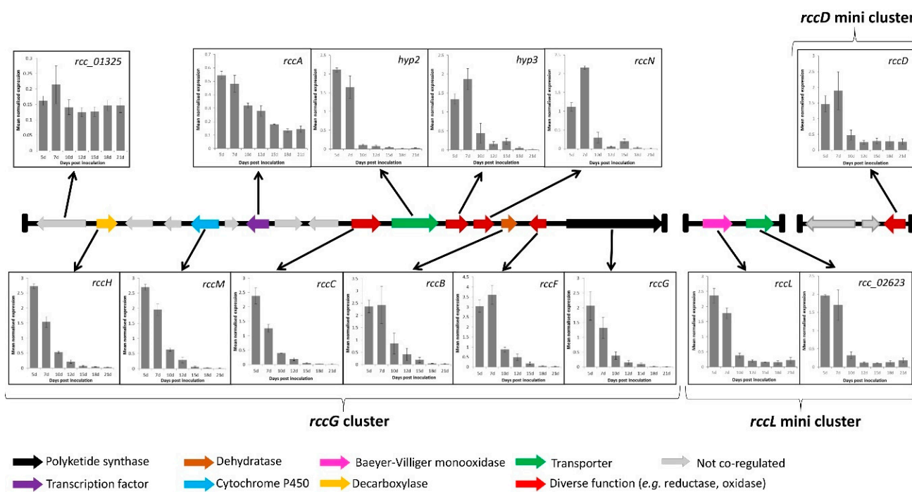
Figure 4. Expression of genes in the rubellin candidate biosynthetic cluster during disease development in artificially inoculated barley seedlings. Disease development was previously described by Dussart et al. [26]. Early symptoms appearance was recorded at 7 dpi, with typical lesions being clearly visible after 10 dpi. Genes represented in grey did not appear to be coregulated based on the RNA-seq data published by McGrann et al. [43]. The expression profile of gene Rcc_01325 was used to validate the results of the RNA-seq data. Data show mean normalised expression value \pm standard error of three independent experiments.
