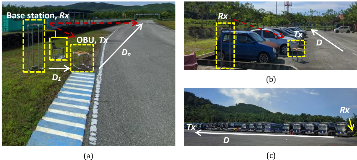
Figure 1. Measurement Campaign at (a) UniMAP Racing Circuit, (b) student's hostel car park, (c) UniMAP bus station with R_x is referring to Base Station, T_x as Mobile Unit and D is distance.
