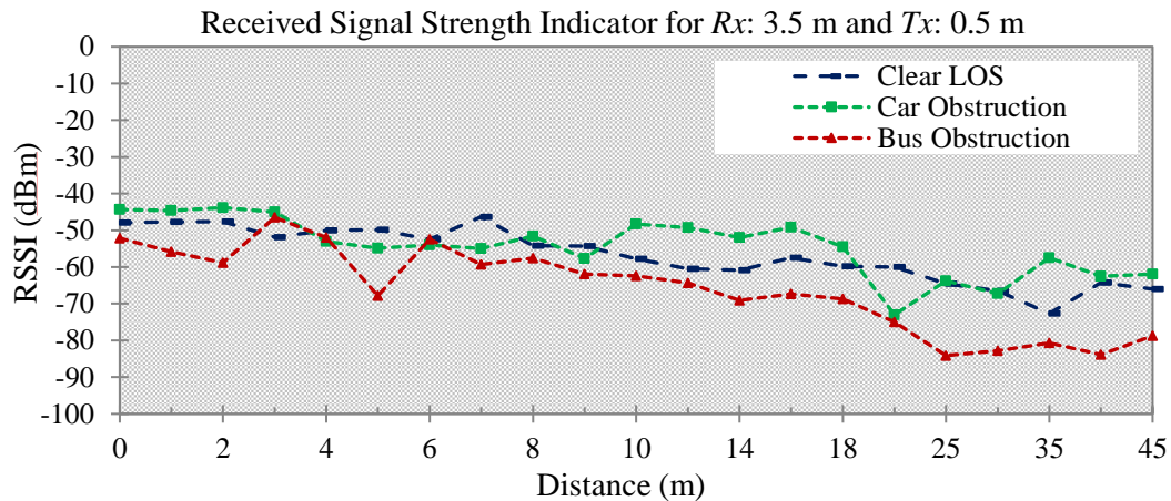
Figure 3. Attenuation profile for LOS, car and bus obstruction at 3.5 x 0.5 m antenna height.
