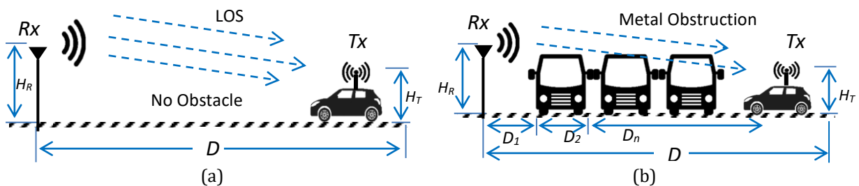
Figure 2. Channel measurement setup under (a) LOS scenario with free-way road and (b) NLOS scenario consisting metal object in between transmitting, T_x and receiving, R_x antennas.
