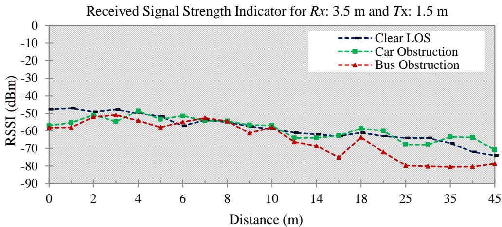
Figure 4. Attenuation profile for LOS, car and bus obstruction at 3.5 x 1.5 m antenna height.
