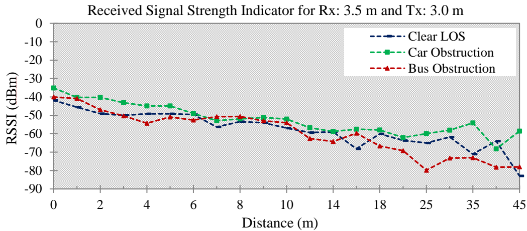
Figure 5. Attenuation profile for LOS, car and bus obstruction at 3.5 x 3.0 m antenna height.
