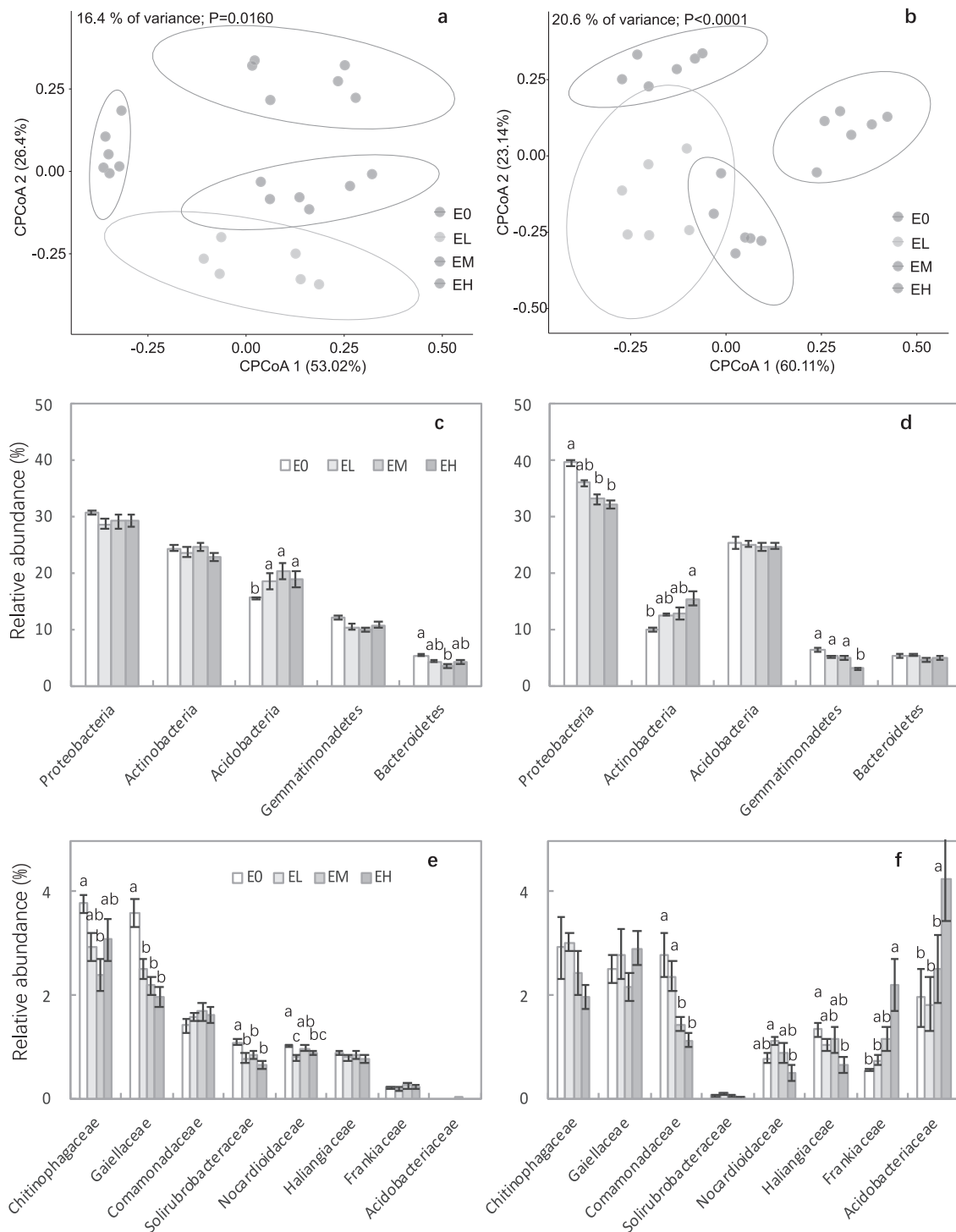
Fig. 2 Soil bacterial composition as affected by soil erosion at the Fuxian and Nenjiang sites. Constrained Principle Coordinate Analysis (CPCoA) plot of Bray-Curtis distances among soil erosion treatments ( a : Fuxian; b : Nenjiang), the relative abundance of the dominant bacterial phyla ( c : Fuxian; d : Nenjiang) and of bacteria at family level that were significantly affected by soil erosion at any of the two sites ( e : Fuxian; f : Nenjiang). The results of similarity
