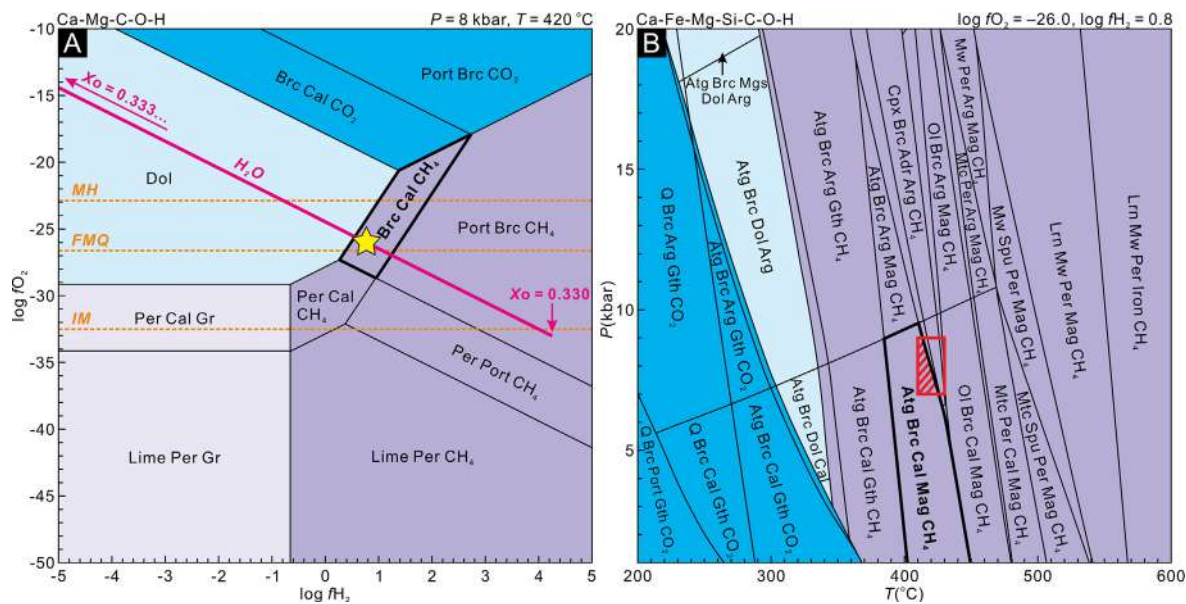
Fig. 7. (A) Stabilities of phases under variable f\text{O}_2 and f\text{H}_2 conditions in the Ca-Mg-C-O-H system (with fixed Ca:Mg:C of 1:1:2 in molar ratio) at 8 kbar and 420 °C. The orange dashed lines show \log f\text{O}_2 of magnetite-hematite (MH), fayalite-magnetite-quartz (FMQ), and iron magnetite (IM) buffers calculated at 8 kbar and 420 °C. The pink solid line represents the thermodynamically calculated model of slightly reduced \text{H}_2\text{O} at X_{\text{O}} greater than or equal to 0.330 but less than 0.333... in the H-O system (star: X_{\text{O}} = 0.3333323 , corresponding to y_{\text{H}_2\text{O}} = 0.9999995 and y_{\text{H}_2} = 0.0000005 ). (B) The P - T pseudosection displaying diverse phase assemblages in the Ca-Fe-Mg-Si-C-O-H system at \log f\text{O}_2 = -26.0 and \log f\text{H}_2 = 0.8 . The rectangle confines P - T conditions for the onset of retrograde serpentinization in the Tianshan (7.9 kbar and 410–430 °C; Li et al., 2007, 2010).
