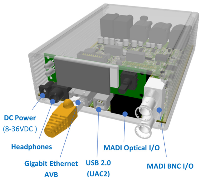
Fig. 4. Input/output connectivity of the A 2 B-DSP board, front view.
