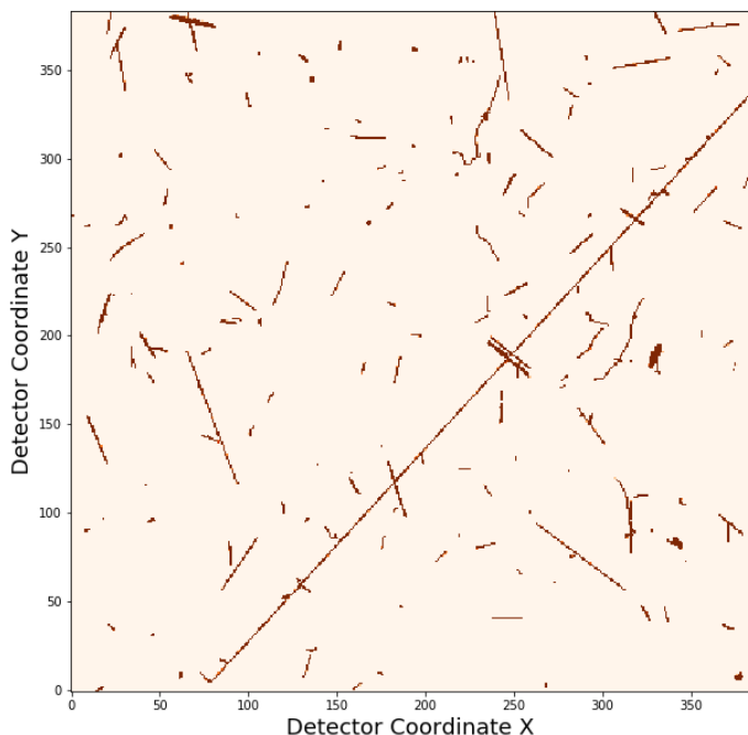
Fig. 5. Stack of numerous CCD raw frames from all TM7s taken in orbit. This shows the variety of cosmic radiation particles hitting the cameras at all times, which in orbit amount to typically one to three per readout frame every 50 ms.
