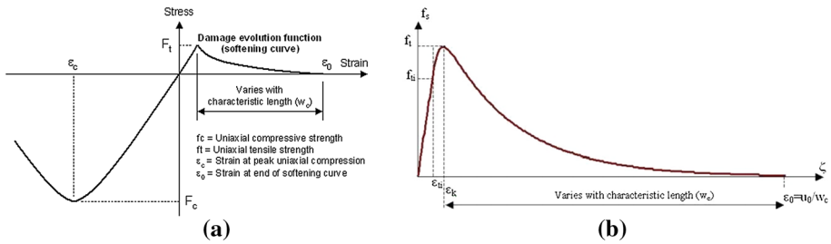
Fig. 3 Model C: a Stress/strain curve for smoothed multi-crack concrete model and b damage evolution function (softening curve)
