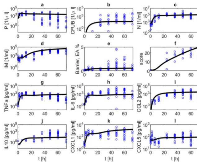
Fig 4. Comparison of model and data for a scenario of infection with 5 \cdot 10^6 Streptococcus pneumoniae without treatment. Time series of pneumococcal population in BAL (a) and blood (b), neutrophils in BAL (c), inflammatory macrophages in BAL (d), barrier function (e), histologic score (f), TNF- \alpha in BALF (g), IL-6 in BALF (h), CCL2 in BALF (i), IL-10 in BALF (j), CXCL1 in BALF (k) and CXCL5 in BALF (l) without antibiotic treatment are displayed. The solid black curve represents simulation results. Circles represent data points. In this scenario, the immune system is not able to remove the infection resulting in increasing numbers of immune cells, pro-inflammatory cytokines, barrier failure and bacteremia.
