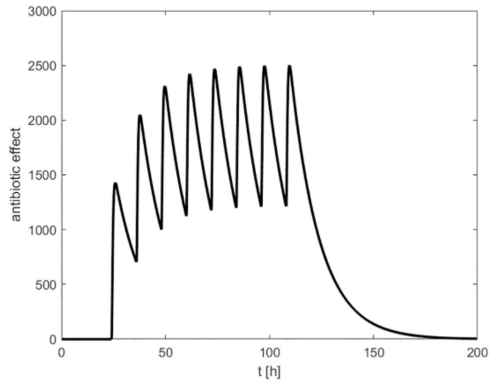
Fig 2. Antibiotic therapy. In this example, the antibiotic effect A(t) of repetitive drug administrations in time intervals of 12 hours is shown. Therapy starts 24 hours after infection and stops after 8 injections.
