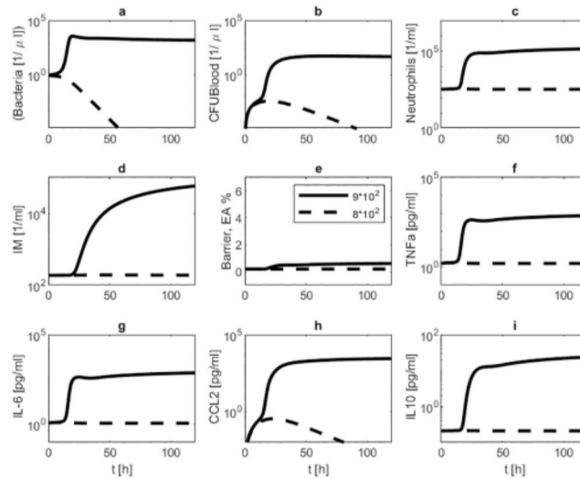
Fig 3. Model behaviour in dependence on initial bacterial load. We present simulation results of infections with 8 \cdot 10^2 (dotted line) respectively 9 \cdot 10^2 (solid line) seeded Streptococcus pneumoniae without treatment. Time series of pneumococcal population in BAL (a) and blood (b), neutrophils in BAL (c), inflammatory macrophages in BAL (d), barrier function (e), TNF- \alpha in BALF (f), IL-6 in BALF (g), CCL2 in BALF (h) and IL-10 in BALF (i) are displayed. The lower infectious dose results in cure while the larger infectious dose leads to disseminated disease.
