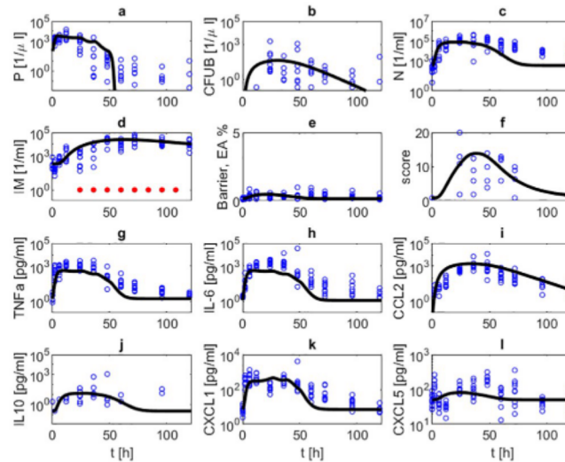
Fig 5. Infection with 5 \cdot 10^6 Streptococcus pneumoniae treated with ampicillin (0.4 mg/mouse) every 12h, starting at 24h. We compare results of model simulation with data under antibiotic treatment. Time series of pneumococcal population in BAL (a) and blood (b), neutrophils in BAL (c), inflammatory macrophages in BAL (d), barrier function (e), histologic score (f), TNF- \alpha in BALF (g), IL-6 in BALF (h), CCL2 in BALF (i), IL-10 in BALF (j), CXCL1 in BALF (k) and CXCL5 in BALF (l) are displayed. The solid black curve represents simulation results. Blue circles represent data. Red dots represent the time points of antibiotic treatment. Treatment results in eradication of bacteria from alveolar spaces and blood. Immune cells, cytokine levels and barrier function also normalize except for macrophages staying elevated during observation period.
