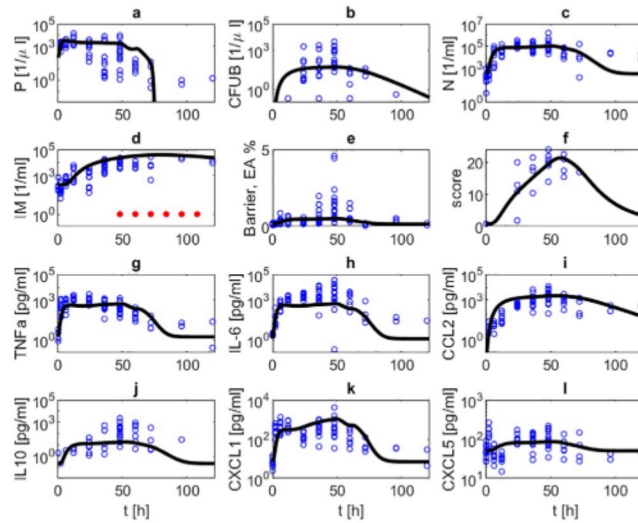
Fig 6. Infection with 5 \cdot 10^6 Streptococcus pneumoniae treated with ampicillin (0.4 mg/mouse) every 12h, starting at 48h. We compare results of model simulation with data under antibiotic treatment. Time series of pneumococcal population in BAL (a) and blood (b), neutrophils in BAL (c), inflammatory macrophages in BAL (d), barrier function (e), histologic score (f), TNF- \alpha in BALF (g), IL-6 in BALF (h), CCL2 in BALF (i), IL-10 in BALF (j), CXCL1 in BALF (k) and CXCL5 in BALF (l) are displayed. The solid black curve represents simulation results. Blue circles represent data. Red dots represent the time points of antibiotic treatment. Dynamics of state parameters are similar to that of antibiotic treatment starting at 24h but with some delay.
