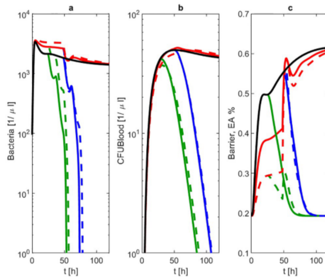
Fig 9. Prediction scenarios. We simulated the outcome of combined 20 mg/kg NOX-D19 and antibiotic treatment starting 24h (green dashed line) or 48h (blue dashed line) after infection and compared the results with no treatment (black solid line), antibiotic treatment alone 24h (green solid line) or 48h (blue solid line) after infection or 2 mg/kg (red solid line) respectively 20 mg/kg (red dashed line) NOX-D19 alone. Time series of pneumococcal population in BAL (a) and blood (b) and barrier function (c) are displayed. Cure is only achieved in scenarios with antibiotic treatment. Bacteremia is smallest in case of 20 mg/kg NOX-D19 combined with early antibiotic treatment.
