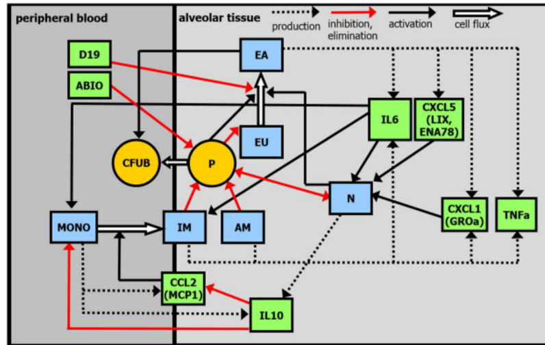
Fig 1. Structure of the model. Compartments: pneumococci in lungs (P), pneumococci in peripheral blood (CFUB), unaffected epithelial/endothelial cells (EU), affected epithelial/endothelial cells (EA), alveolar macrophages (AM), inflammatory macrophages (IM), neutrophils (N), monocytes in peripheral blood (MONO), cytokine / chemokine network comprising IL-6, IL-10, CCL2, CXCL1, CXCL5 and TNF \alpha . ABIO denotes the antibiotic therapy. D19 represents the effect of NOX-D19 treatment.
