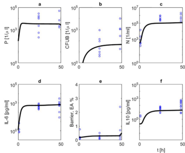
Fig 8. (Treatment with 20 mg/kg NOX-D19). We compare results of model simulation (solid black curve) with data under 20 mg/kg NOX-D19 treatment. Time series of pneumococcal population in BAL (a) and blood (b), neutrophils in BAL (c), IL-6 in BALF (d), barrier function (e) and IL-10 in BALF (f) are displayed. Circles represent data points [2]. NOX-D19 is applied 0 and 24 hours after infection. NOX-D19 alone is insufficient to eradicate the disease but stabilizes the barrier function.
