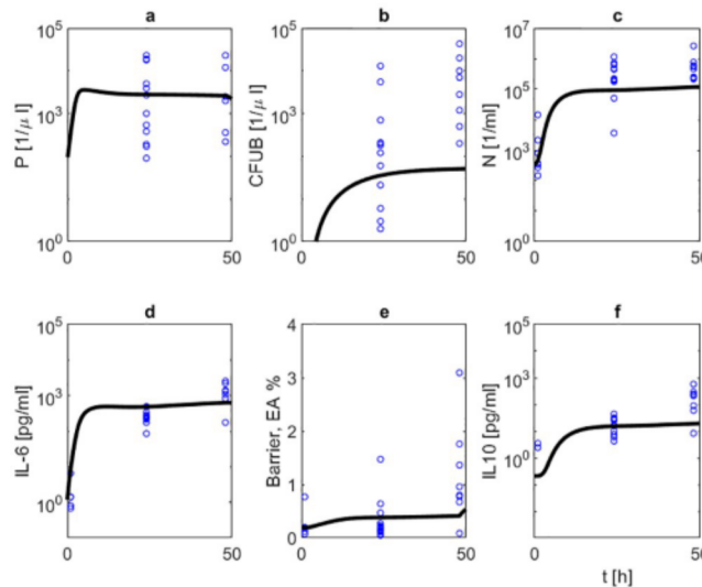
Fig 7. (Treatment with 2 mg/kg NOX-D19). We compare results of model simulation (solid black curve) with data under 2 mg/kg NOX-D19 treatment. Time series of pneumococcal population in BAL (a) and blood (b), neutrophils in BAL (c), IL-6 in BALF (d), barrier function (e) and IL-10 in BALF (f) are displayed. Circles represent data points [2]. NOX-D19 is applied 0 and 24 hours after infection. NOX-D19 treatment alone does not help to eradicate the disease but stabilizes the barrier function.
