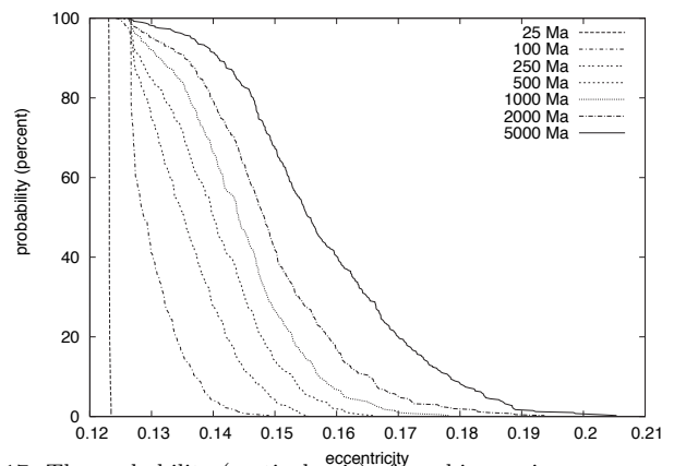
Figure 17: The probability (vertical axis) of reaching a given eccentricity (horizontal axis) after a specified time is given by the different curves, for 25, 100, 250, 500, 1000, 2000, 5000 Myr. The estimate is obtained with 403 different orbital solutions of the secular equations.
