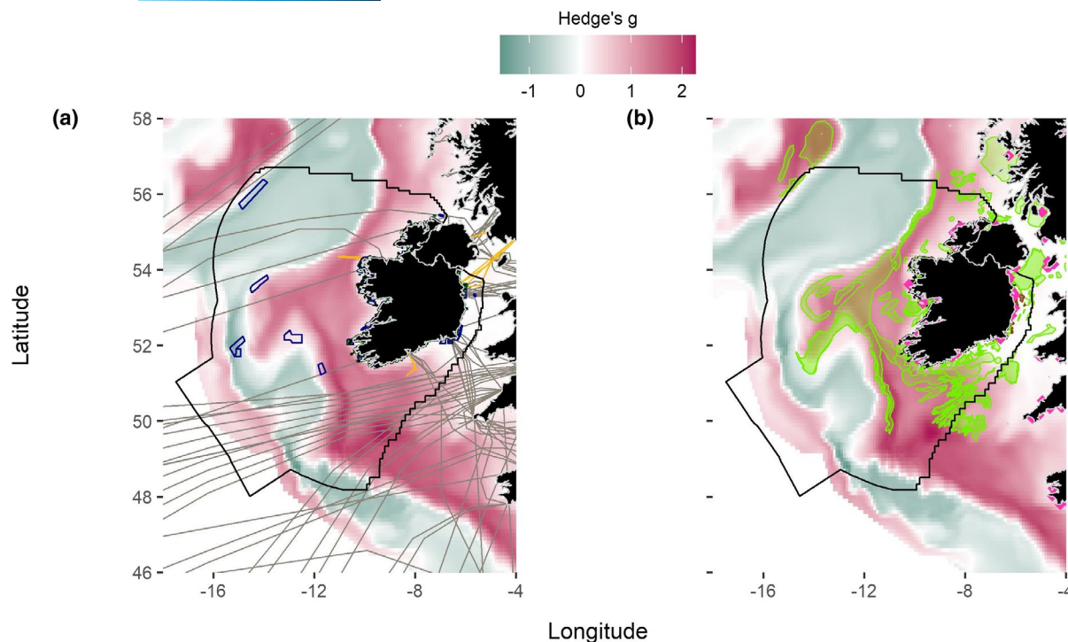
FIGURE 6 Climate-driven changes in the distribution of areas potentially accumulating organic carbon on the seabed, between 2011–2020 and 2040–2049, based on the calculation of Hedges' g (Section 2), under RCP8.5. The background colour green indicates areas where organic carbon accumulation decreases by 2040–2049, given the basin-scale expectation of decreased productivity and increased stratification, while pink indicates the opposite trend (increased supply of organic carbon for potential carbon sequestration on the seabed). (a) areas of the seabed where, due to already existing infrastructure or restrictions, activities that perturb the ability of the seabed to store carbon may already be limited, such as I SACs and SPAs (dark blue and dark green lines respectively), undersea cables (grey) and pipelines (yellow). (b) areas where activities from sectors that will negatively affect the ability of the seabed to store carbon take place, including benthic/demersal fisheries (pale green shading), potential sites for aggregate extraction (brown shading), and ongoing capital and maintenance dredging (pink diamonds)
