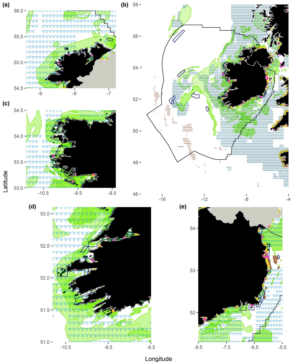
FIGURE 4 Vulnerabilities that arise from climate change for the spatial management of Irish marine conservation sites in 2040–2049, under RCP8.5, given the distribution of habitat-degrading, spatially managed sectors. The colour of triangles denotes CC hotspots (blue) or bright spots (red) in the time period and scenario analysed, with no triangles denoting CC refugia. Upward triangles reflect results from the analysis of pelagic datasets, and inverted triangles indicate the results of benthic and demersal datasets. Overlapping triangles indicate where hotspots and/or bright spots occur in both pelagic and benthic/demersal analyses. Dark blue and dark green outlines indicate the locations of Special Areas of Conservation and Special Protection Areas respectively. Areas shaded in pale green are the locations of fishing grounds. Brown shading indicates areas that could be used for aggregate extraction. Yellow squares are areas of sewage inflow, and pink diamonds are areas where capital and maintenance dredging takes place
