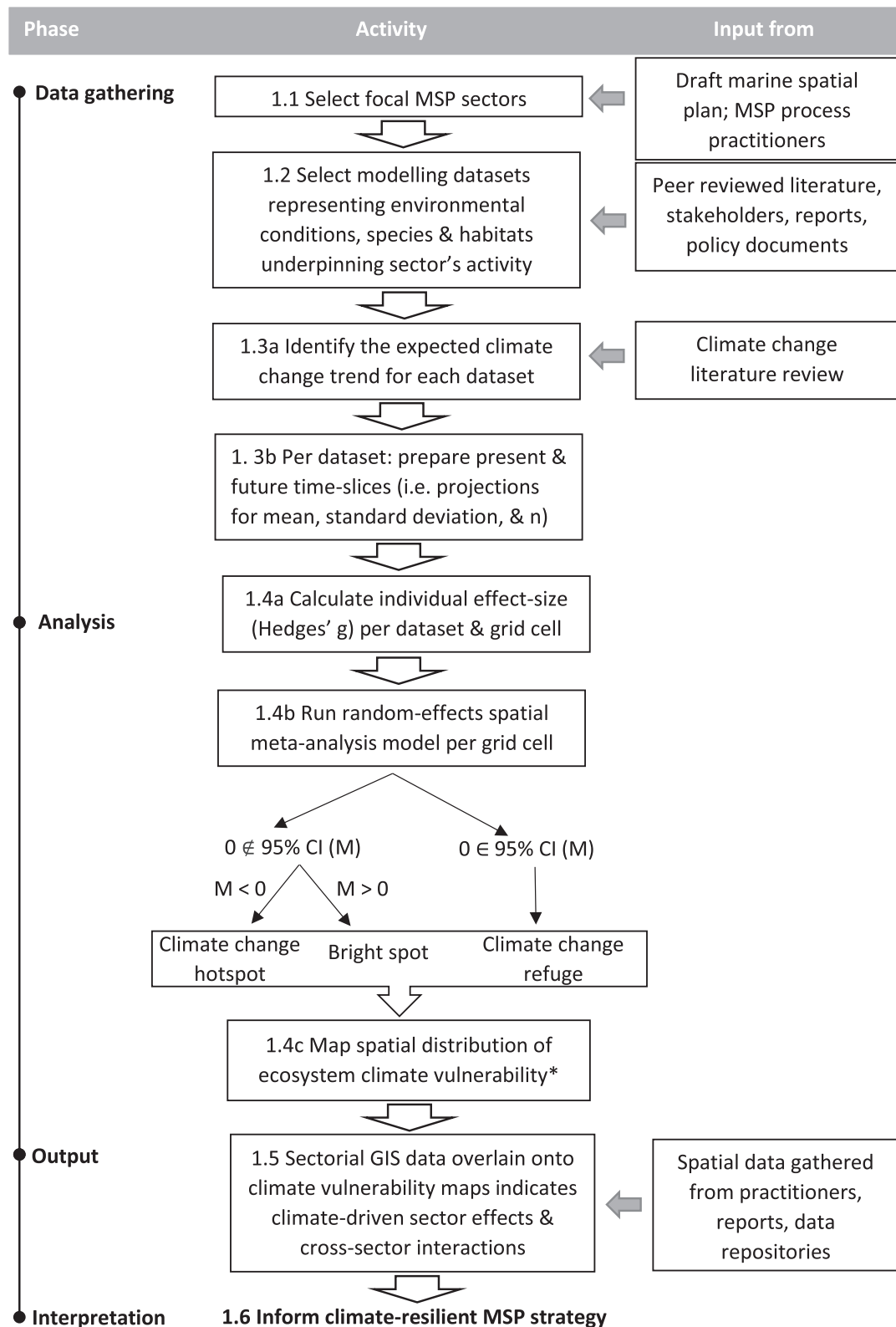
FIGURE 1 Schematic representation of the analytical approach employed, from data gathering, to advice. Please refer to Section 2. Further technical recommendations about each step of this approach are made in Supplementary Information
