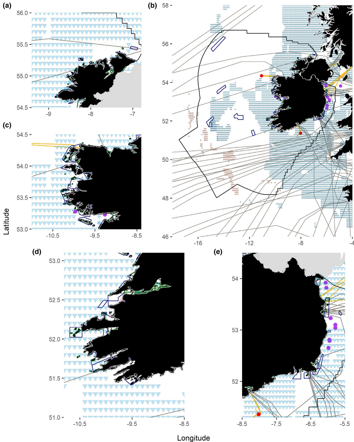
FIGURE 5 Opportunities that arise from climate change for the spatial management of Irish marine conservation sites in 2040–2049, under RCP8.5, given the distribution of other sectors that limit destructive extractive practices. The colour of triangles denotes CC hotspots (blue) or bright spots (red) in the time period and scenario analysed, with no triangles denoting CC refugia. Upward triangles reflect results from the analysis of pelagic datasets, and inverted triangles indicate the results of benthic and demersal datasets. Overlapping triangles indicate where hotspots and/or bright spots occur simultaneously in pelagic and benthic/demersal analyses. Dark blue and dark green outlines indicate the locations of Special Areas of Conservation and Special Protection Areas respectively. Grey lines are the (schematic) locations of undersea cables, yellow lines are the locations of undersea pipelines. Purple circles are the locations of planned, approved, under construction or active offshore wind installations and red circles are oil and gas platforms
