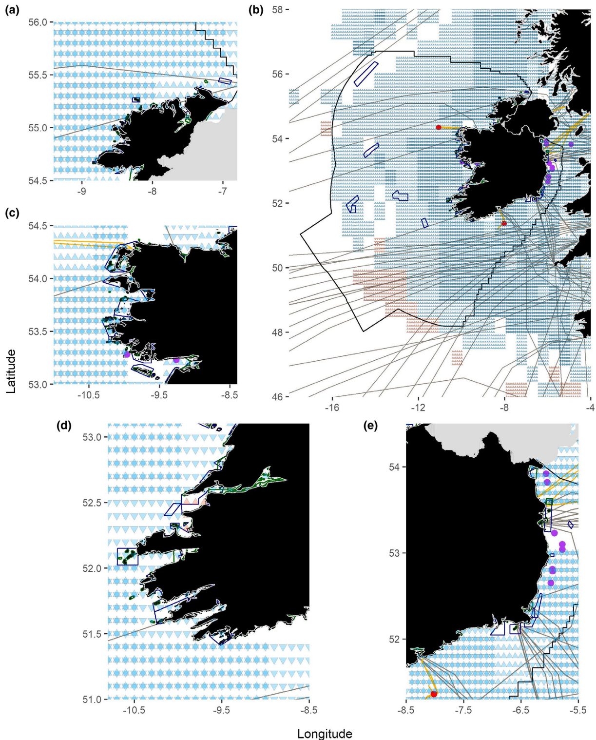
FIGURE 3 Opportunities that arise from climate change for the spatial management of Irish pelagic and benthic/demersal fisheries in 2040–2049, under RCP8.5, given the distribution of other sectors that limit destructive extractive practices. The colour of triangles denotes CC hotspots (blue) or bright spots (red) in the time period and scenario analysed, with no triangles denoting CC refugia. Upward triangles reflect results from the analysis of pelagic datasets, and inverted triangles indicate the results of benthic and demersal datasets. Overlapping triangles indicate where hotspots and/or bright spots occur simultaneously in pelagic and benthic/demersal analyses. Dark blue and dark green outlines indicate the locations of Special Areas of Conservation and Special Protection Areas respectively. Grey lines are the (schematic) locations of undersea cables, yellow lines are the locations of undersea pipelines. Purple circles are the locations of planned, approved, under construction or active offshore wind installations and red circles are oil and gas platforms
