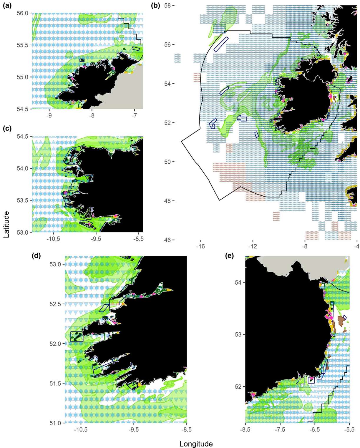
FIGURE 2 Vulnerabilities that arise from climate change for the spatial management of Irish pelagic and benthic/demersal fisheries in 2040–2049, under RCP8.5, given the distribution of other habitat-degrading spatially managed sectors. The colour of triangles denotes CC hotspots (blue) or bright spots (red) in the time period and scenario analysed, with no triangles denoting CC refugia. Upward triangles reflect results from the analysis of pelagic datasets, and inverted triangles indicate the results of benthic and demersal datasets. Overlapping triangles indicate where hotspots and/or bright spots occur in both pelagic and benthic/demersal analyses. Dark blue and dark green outlines indicate the locations of Special Areas of Conservation and Special Protection Areas respectively. Areas shaded in pale green are the locations of fishing grounds. Brown shading indicates areas that could be used for aggregate extraction. Yellow squares are areas of sewage inflow, and pink diamonds are areas where capital and maintenance dredging takes place
