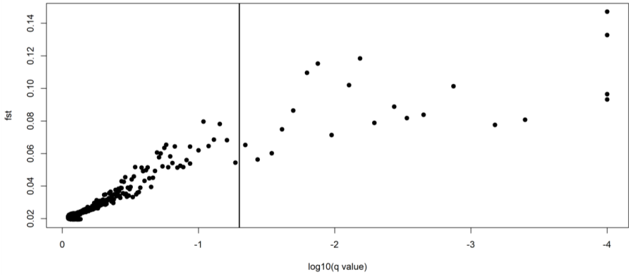
Supplementary figure 14: Detection of outlier loci in Bayescan, using a dataset of 493 Dipturus batis from 6 sampling locations, genotyped at 6,350 loci. Twenty-one loci under putative positive selection are shown to the right of the FDR threshold of 0.05 (vertical line).
