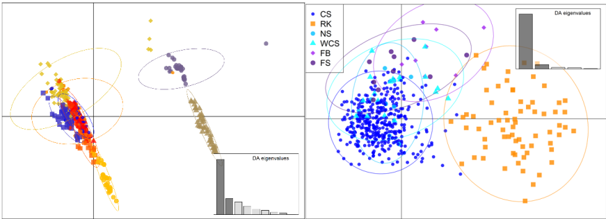
Supplementary figure 8: Discriminant analysis of principal components (DAPC) depicting the diversity between 493 blue skates in 10 inferred groups (left) and 6 groups defined by geographical location (right), using only 21 outlier loci. DAPC results were plotted using all 21 PCs (explaining 100% of variance), after retaining 9 and 5 discriminant functions of inferred and pre-defined groups respectively. 95% inertia ellipses are shown. Site names are abbreviated for the Celtic Sea (CS), West Coast Scotland (WCS), Northern Scotland (NS), Rockall (RK), the Faroe Bank (FB), and the Faroe Shelf (FS).
