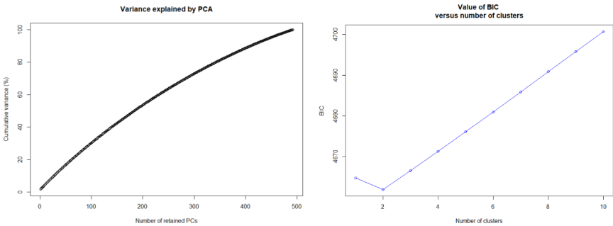
Supplementary figure 7: Analysis plots for a discriminant analysis of principal components (DAPC) on 6,350 SNPs from 493 individuals of Dipturus batis , using the find.clusters function implemented in the R package adegenet . The figures depict the cumulative variance (%) explained by 493 principal components, and the Bayesian Information Criterion (BIC) for each inferred number of clusters ranging from 1 to 10.
