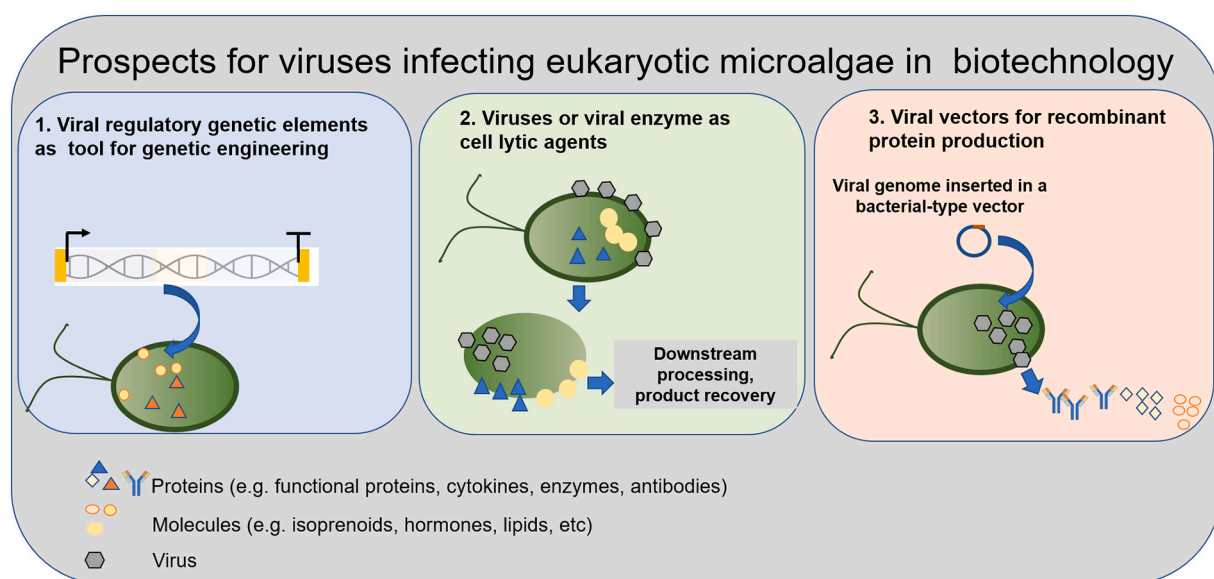
Fig. 1. Schematic representation of the major prospects for viruses infecting microalgae in biotechnology. (1) Viral genetic regulatory elements (e.g. promoters, terminators, ribosome binding sites, transcription enhancers, etc.) can be predicted and isolated from the viral genomes, and used as gene expression tools in genetic and metabolic engineering; (2) viruses or viral enzymes capable of degrading cell walls can be used as lytic agents, helping the recovery of cellular products in biorefinery; (3) viral vectors can be generated and engineered for the production of recombinant protein and biopharmaceuticals.
