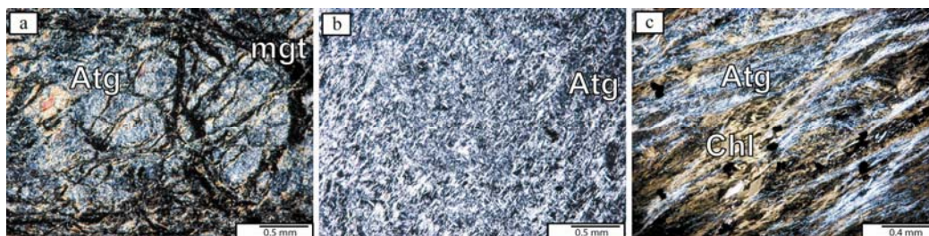
Figure 8. Photomicrographs of serpentinites from Monviso under cross-polarized light after Auzende et al. (2005). a) Interpenetrative antigorite surrounded by fine grained magnetite that outlines the pseudomorph of olivine (Sample 624-2 : Viso Mozzo), b) Typical antigorite interpenetrative texture in metabasalt? (Sample 623-3 : Lago Superiore), c) Sheared serpentinite where antigorite and chlorite (Chl) define the foliation Postkinematic chlorite crystals cut the foliation (Sample 625-6 : Lago Superiore).
