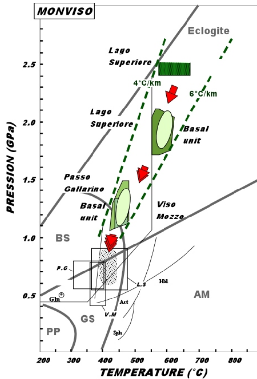
Figure 7 : P-T paths of eclogitic units in Monviso, showing that different units show similar retrogression paths under blueschist facies conditions. Note that the P-T paths yield the geothermal gradients of 4 to 6°/km, typical of subduction zone conditions.
