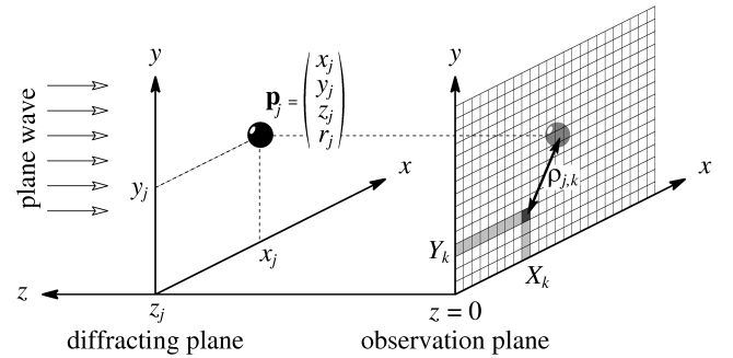
Fig. 2. Notations used in the hologram model. The parameters \mathbf{p}_j = \{x_j, y_j, z_j, r_j\} are the position and radius of the j -th particle, (X_k, Y_k) is the location of the k -th pixel and \rho_{j,k} is the distance between the projection of the j -th particle on the detector and the k -th pixel.
