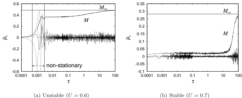
FIG. 1: Stationarity check for initial distributions with power-law tails. Note the logarithmic scale for the rescaled time \tau = t/N . Panel (a) presents the unstable case U = 0.6 while panel (b) the stable one U = 0.7 . The three curves \dot{\mu}_n ( n = 1, 2, 3 ) are reported in both panels. Their vertical scales are multiplied by 100 for graphical purposes. Curves and horizontal lines indicated by symbols M and M_{eq} represent respectively temporal evolutions of the magnetization and its equilibrium value. All numerical curves are obtained by averaging 20 different numerical simulations for N = 10^4 .
