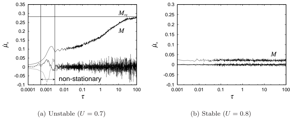
FIG. 3: Stationarity check for gaussian initial distributions with N = 10^4 . Note the logarithmic scale for the rescaled time \tau = t/N . Panel (a) presents the unstable case U = 0.7 while panel (b) the stable one U = 0.8 . The three curves \dot{\mu}_n ( n = 1, 2, 3 ) are reported in both panels. Their vertical scales are multiplied by 100 for graphical purposes. Curves indicated by symbol M represent the temporal evolutions of the magnetization. In panel (a), the horizontal line indicated by M_{eq} represents the equilibrium value, while in panel (b), the equilibrium value is zero. All numerical curves are obtained by averaging 20 different numerical simulations.
