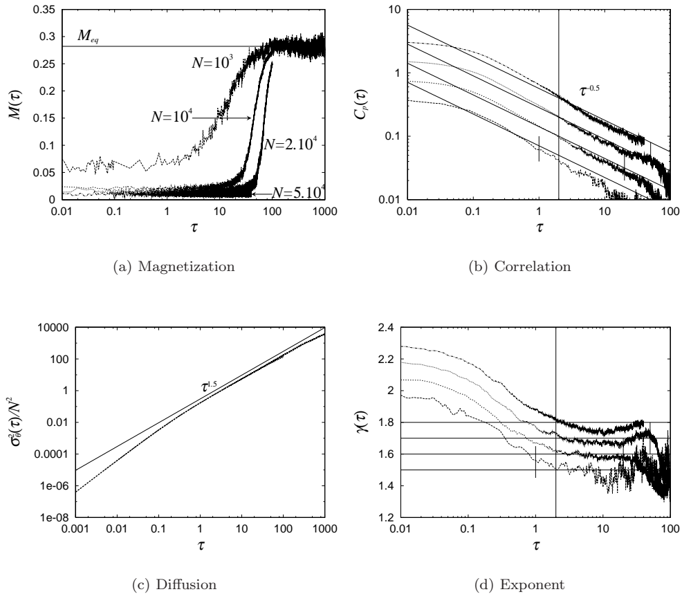
FIG. 2: Check of the theoretical prediction for stable initial distributions with power-law tails, in the case U = 0.7 . Points are numerically obtained by averaging 20, 20, 10 and 5 realizations for N = 10^3, 10^4, 2.10^4 and 5.10^4 respectively. Panel (a) shows temporal evolution of magnetization in the scale time \tau = t/N . The take-off times of M are estimated as \tau_1 = 1, 20 and 50 for N = 10^3, 10^4 and 2.10^4 respectively, and \tau_2 are marked in panel (b) and (d). No take-off for N = 5.10^4 is observed in this computing time. The horizontal line represents the equilibrium value of M . In panel (b), four curves represent the correlation functions of momenta, while the straight lines with the slope -1/2 represent the theoretical prediction. The curves and the lines are multiplied from the original vertical values by 2, 4 and 8 for N = 10^4, 2.10^4 and 5.10^4 for graphical purposes. The vertical line indicates \tau_1 = 2 from which the valid time region of the theory starts. Similarly, panel (c) presents the diffusion of angles, while the straight line with the slope 3/2 is theoretically predicted. The four curves for the four different values of N are reported and almost collapse. Finally, panel (d) shows the temporal evolution of the instantaneous exponent \gamma , defined in Eq. (8), and \gamma stays around the theoretically predicted value 3/2 in the time region \tau_1 < \tau < \tau_2 . The values 0.1, 0.2 and 0.3 are added in vertical values for N = 10^4, 2.10^4 and 5.10^4 respectively for graphical purposes.
