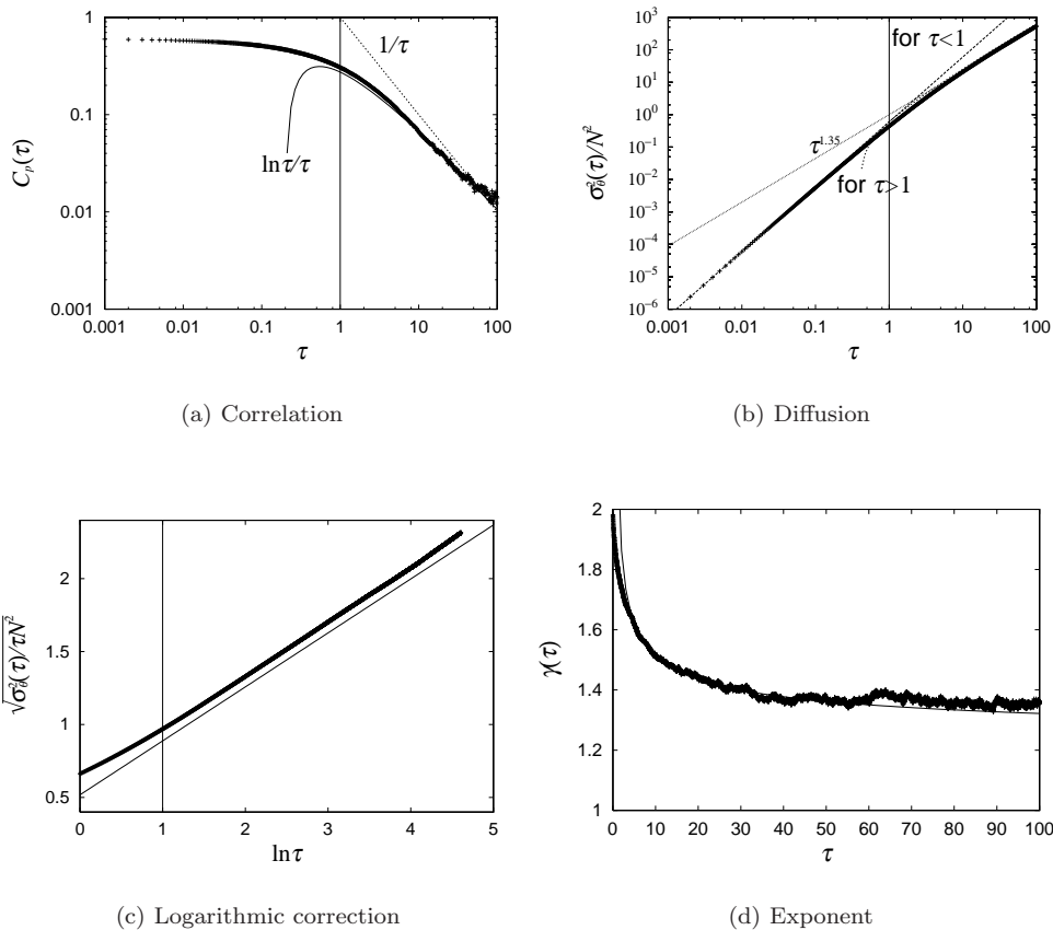
FIG. 4: Check of the theoretical prediction for gaussian stable initial distributions in the case U = 0.8 with N = 10^4 . Points are numerically obtained by averaging 20 realizations. In panel (a), the symbols show the correlation function of momenta. The theoretical prediction, \ln \tau/\tau , is a better approximation than the simpler law 1/\tau . Panel (b) presents the diffusion of angles. Although the diffusion is normal, the straight line \tau^{1.35} wrongly suggests that it is not. See text for explanations and details. Panel (c) shows the quantity \sqrt{\sigma_\theta^2(\tau)/(\tau N^2)} as a function of \ln \tau to confirm the logarithmic correction of the diffusion. The straight line is a guide for the eyes. Finally, panel (d) presents the temporal evolution of the instantaneous exponent \gamma . The dashed line corresponds to relation (12).
