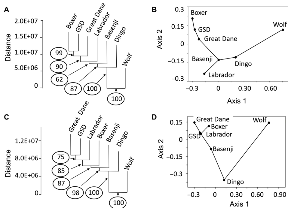
Fig. 3. Phylogenetic and ordination analyses from indels and SNVs of seven canines. (A) Phylogenetic tree from indels with bootstrapping (percentages of times that node appeared in 500,000 bootstraps). (B) Ordination analyses of first two axes from nonmetric multidimensional scaling from indels. (C) Phylogenetic tree from SNVs with bootstrapping (500,000 bootstraps). (D) Ordination analyses of first two axes from nonmetric multidimensional scaling from SNVs. GSD, German shepherd dog; Wolf, Greenland wolf.
