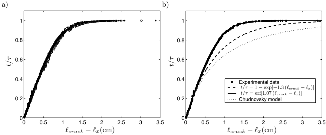
Fig. 7 – On the left: time rescaled by the time left to rupture as a function of l_{crack} - l_x for four experiments performed in the same experimental conditions ( l_i = 1.5\text{cm} , F_c = 900\text{N} , same experiments as for figure 6b) with a change in time and length origins; on the right: time rescaled by the time left to rupture as a function of l_{crack} - l_x for an imposed stress experiment ( l_i = 1.5\text{cm} , F_c = 900\text{N} ) and fits by the Chudnovsky model, the thermal activation model and an error function adjusting the initial velocity.
