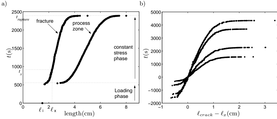
Fig. 6 – On the left: time as a function of both the crack and process zone lengths for an imposed stress experiment ( l_i = 1.5\text{cm} , F_c = 900\text{N} ); on the right: time as a function of l_{crack} - l_x for four experiments performed in the same experimental conditions ( l_i = 1.5\text{cm} , F_c = 900\text{N} ) with a change in time and length origins.
