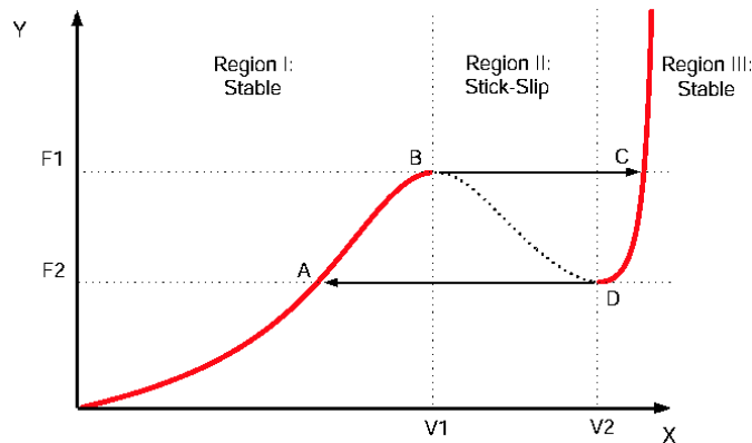
FIG. 1 – Schematic relation between the peeling force f and the peeling velocity v at the peeling crack line. These variables refer to the local dynamics of the peeling point and correspond to the tensile force F and velocity V at the free end of the tape only when the peeling is regular and the peeling angle 90^\circ . The sigmoidal shape is responsible for the hysteretic behavior and therefore for the stick-slip dynamics.
