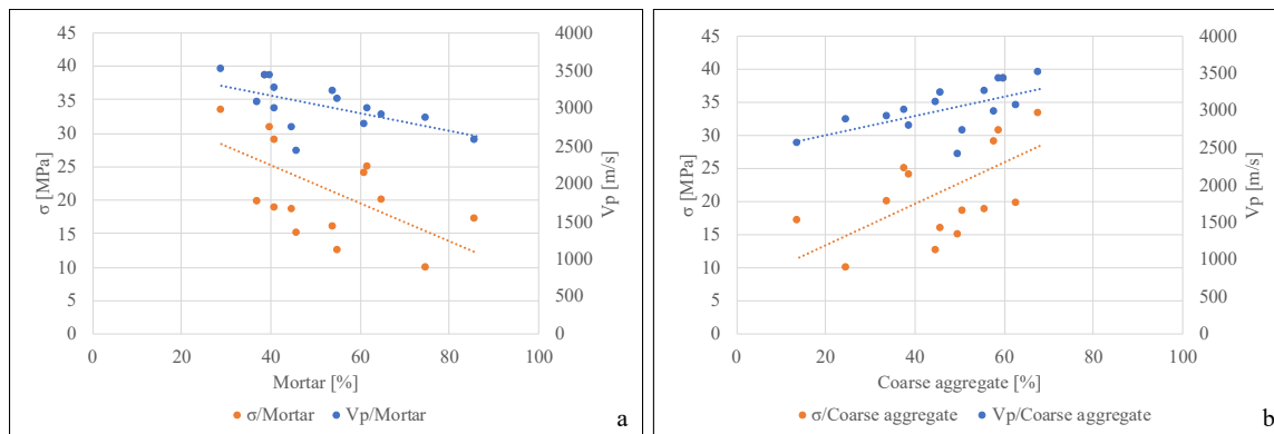
Figure 9. Diagram of correlation between \sigma , V_p , and % of fine portion of core samples (a); \sigma , V_p , and % of coarse aggregate (b).
