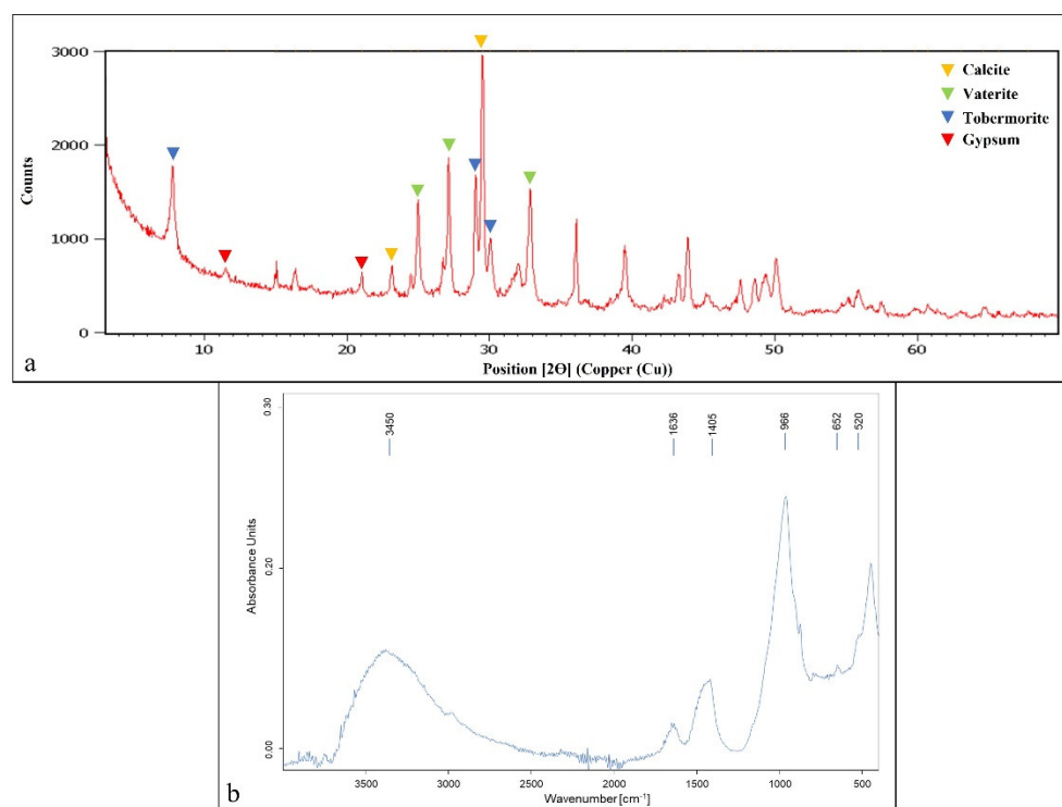
Figure 4. XRD pattern of sample C2-X lump. The most intense peaks for calcite, vaterite, tobermorite and gypsum are indicated (a). FTIR spectra of sample C2-X lump. The vibrational bands of tobermorite are highlighted (b).
