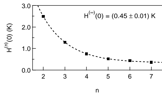
Fig. 7. Experimental H^{(n)}(0) vs. bead position n .
