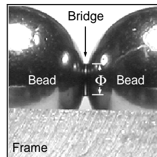
Fig. 11. Photograph of a liquid bridge.
