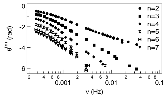
Fig. 6. Phase \theta^{(n)} vs. frequency \nu .
