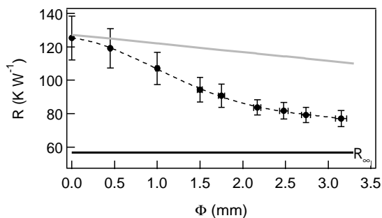
Fig. 13. Resistance R vs. bridge diameter \Phi .
