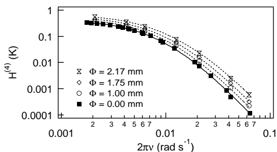
Fig. 12. Amplitude H^{(4)} vs. 2\pi\nu .
