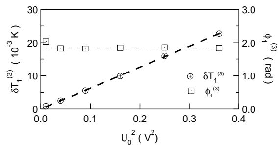
Fig. 3. Amplitude \delta T_1^{(3)} and phase \phi_1^{(3)} vs. U_0^2 .
