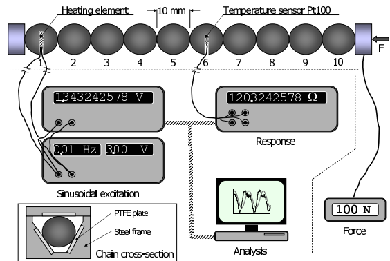
Fig. 1. Sketch of the experimental principle.
