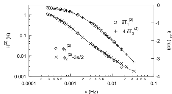
Fig. 4. Experimental H^{(2)} and \theta^{(2)} vs. frequency \nu .
