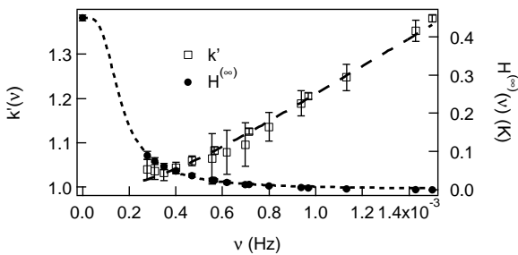
Fig. 9. Asymptotic amplitude H^{(\infty)} and k' vs. \nu .
