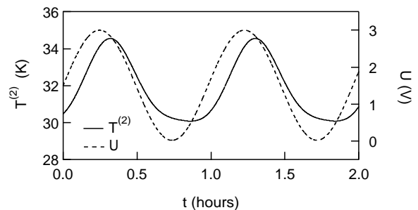
Fig. 2. Experimental T^{(2)} and U vs. time t .
