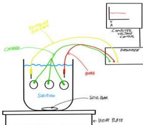
Figure 1. Electrodeposition Experiment Set-Up
