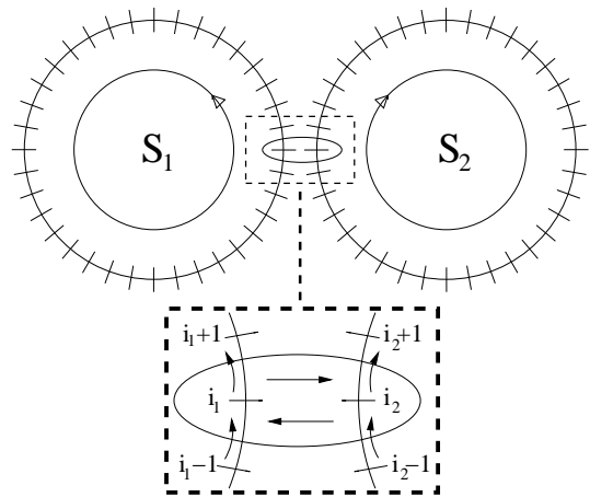
FIG. 1: Illustration of two mass transport models with periodic boundary conditions, connected through a contact made of a single additional link. A zoom over the contact is also shown in the dashed frame; arrows indicate the oriented links through which mass is transported.
