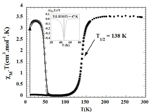
FIG.2. Bottom: Magnetic susceptibility measurements in the form \chi_M \cdot T as a function of the temperature T where \chi_M is the magnetic susceptibility. Data collected at thermal equilibrium are represented by dark circles. Open circles (o) represent data registered after a laser irradiation made at 10 K (schematized by a continuous black arrow) during around one hour, then stopped before a temperature increase ( 0.3 \text{ K} \cdot \text{min}^{-1} ). The black line
