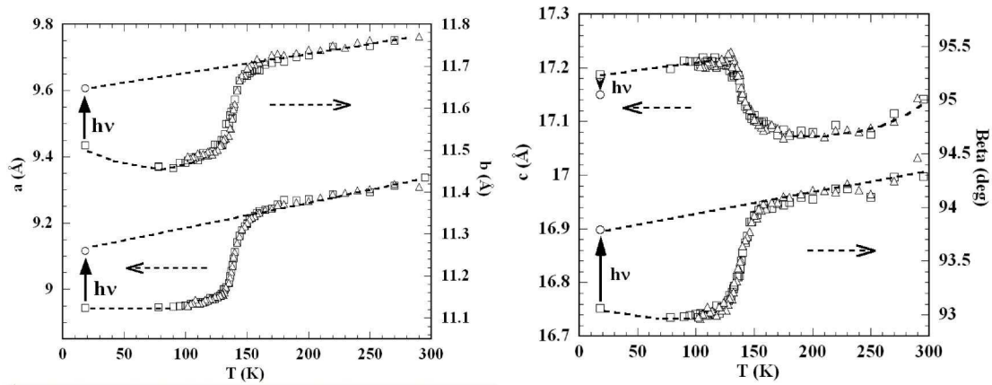
FIG.5. Evolution of the unit-cell parameters as a function of the temperature. Measurements made with increasing temperature are schematized with open triangles ( \Delta ), whereas those made under cooling are schematized with open squares ( \square ). The arrows schematize the laser irradiation ( \lambda = 808 \text{ nm} ) made at 18K. Dashed lines are guides to the eye.
