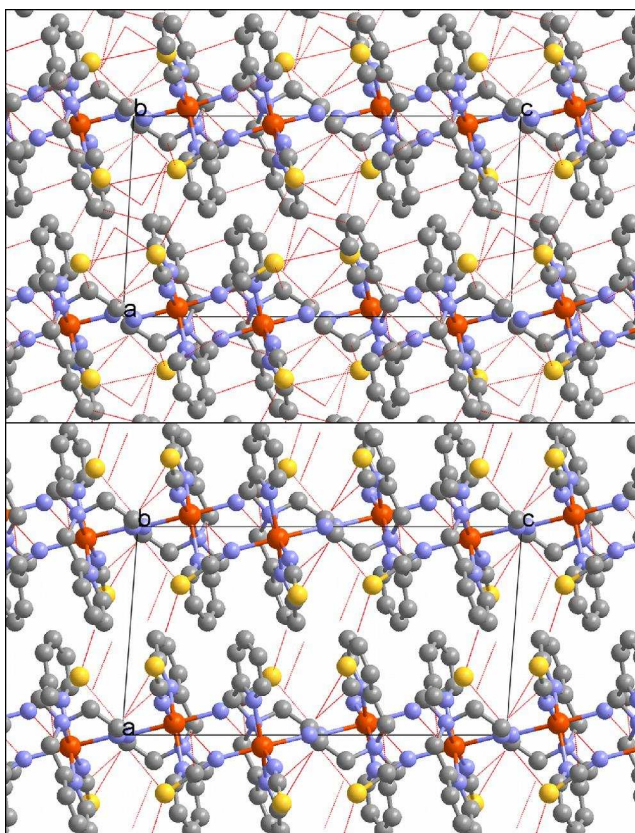
FIG.7. Short intermolecular contacts, defined by distances shorter than the sum of Van Der Waals Radii, from structure resolution at 290 K (down) and 78 K (up). The c axis is the horizontal one, the a axis is the vertical one and the b axis is perpendicular to the figure.
