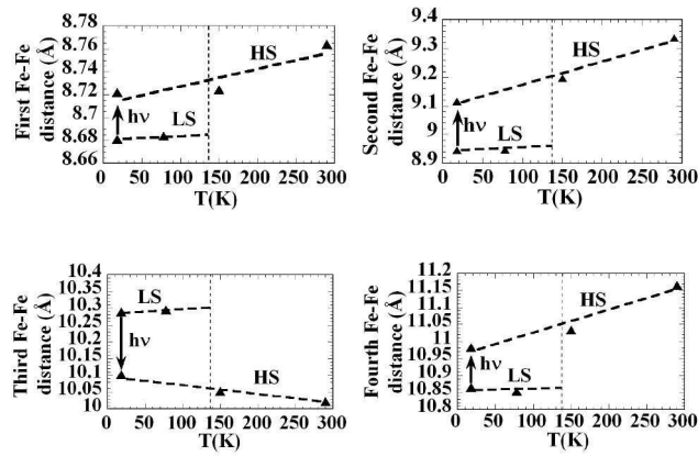
FIG.8. Temperature evolution of the four shortest intermolecular Fe-Fe distances. . The arrows schematize the laser irradiation made ( \lambda = 808 \text{ nm} ) at 18 K. Dashed lines are guides to the eye.
