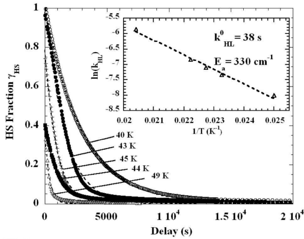
FIG.3. Relaxation of the HS fraction as a function of temperature. Each time, the sample is first irradiated at 10 K where the complete transformation is achieved before the temperature is increased up to the desired temperature and the laser is switched off. The insert illustrates the determination (by the fitted curves in dashed lines) of the kinetic parameters E_a and k_{HL}^\infty defined in the text.
