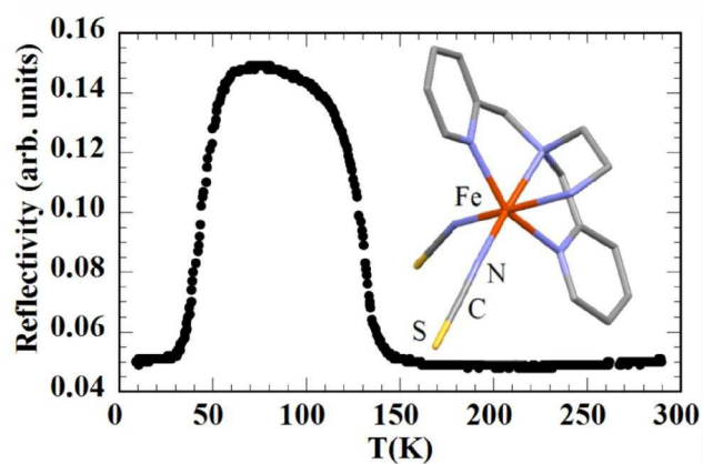
FIG.1. Reflectivity measurements probed at \lambda = 800 \text{ nm} as a function of increasing temperature on [\text{Fe}(\text{DPEA})(\text{NCS})_2] . Insert: schematic representation of the [\text{Fe}(\text{DPEA})(\text{NCS})_2] molecule (Hydrogen atoms are omitted for clarity).
