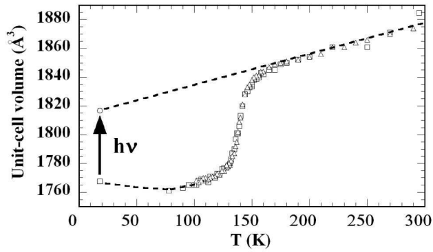
FIG.4. Evolution of the unit-cell volume as a function of the temperature. Measurements made with increasing temperature are schematized with open triangles ( \Delta ), whereas those made under cooling are schematized with open squares ( \square ). The arrow schematizes the laser irradiation ( \lambda = 808 \text{ nm} ) made at 18 K. Dashed lines are guides to the eye.
