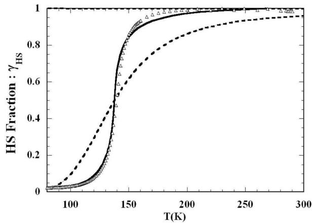
FIG.9. Evolution of the HS molar fraction \gamma_{HS} (shown with \Delta ) as a function of temperature T . The lines represent fitted curves with T_{1/2} fixed to 138 K and \Delta H is taken equal to 6760 \text{ J.mol}^{-1} according to previous experiments 23 : the dashed line is the fit deduced from equation (ii) when the intermolecular interaction term \Gamma = 0 and the continuous line is a similar fit but adjusting a non-zero value for \Gamma = 2042 \pm 94 \text{ J.mol}^{-1} for fitting the experimental data.
